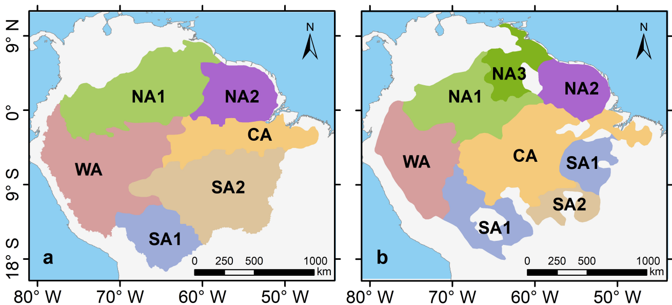
Figure 4. The spatial distribution of (a) K-means clustering analysis map of MTVDI, (b) The seasonality cluster map identified from monthly data of land surface temperature ( T_s ), canopy backscatter from Quick Scatterometer (QSCAT), and reflectance of near-infrared (NIR).
