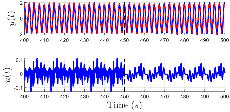
Figure 10: Zoom-in of the identification results obtained following the optimal procedure with c_1 = 1, c_2 = 0 . The probing signal u(t) is plotted in percentages of its nominal value ( i.e. , 0.1 means a 10% deviation of its nominal value).
