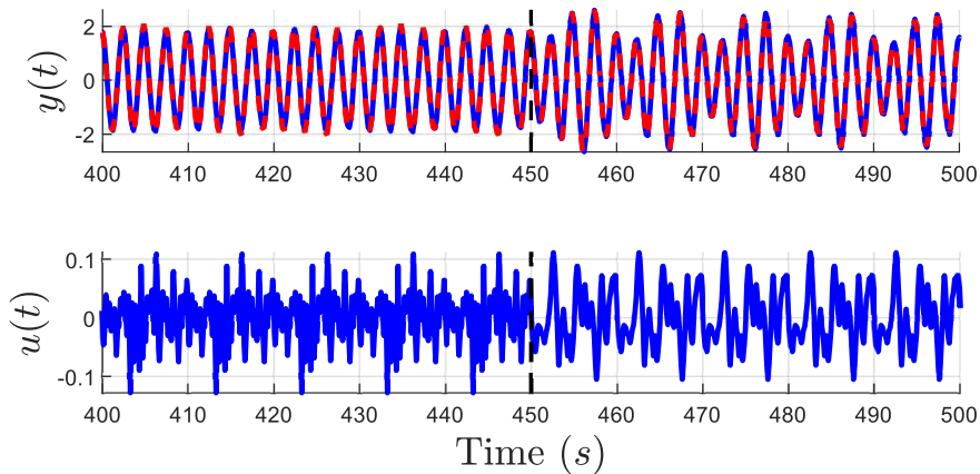
Figure 12: Zoom-in of the identification results obtained following the optimal procedure with c_1 = 3/4, c_2 = 1/4 . The probing signal u(t) is plotted in percentages of its nominal value ( i.e. , 0.1 means a 10% deviation of its nominal value).
