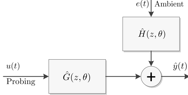
Figure 1: Power system representation as seen in the prediction error system identification method with probing signal u(t) and measurement estimation \hat{y}(t) .
