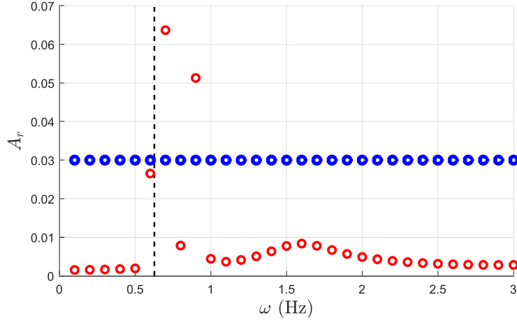
Figure 6: The amplitudes A_r from the base procedure (blue), and optimized ones (red) with c_1 = 1/2, c_2 = 2500 . The vertical dashed line indicates the frequency of the true inter-area mode.
