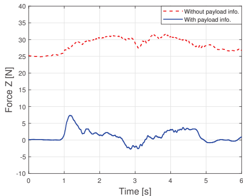
Fig. 4. Comparison of the force applied by the person to move a total load of 3.2\text{kg} with and without the information of the payload in the controller and model.
