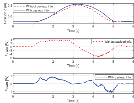
Fig. 5. Comparison of the trajectories performed with and without knowledge of the payload (total load of 3.2\text{kg} ), and the respective power supplied to the system by the person.
