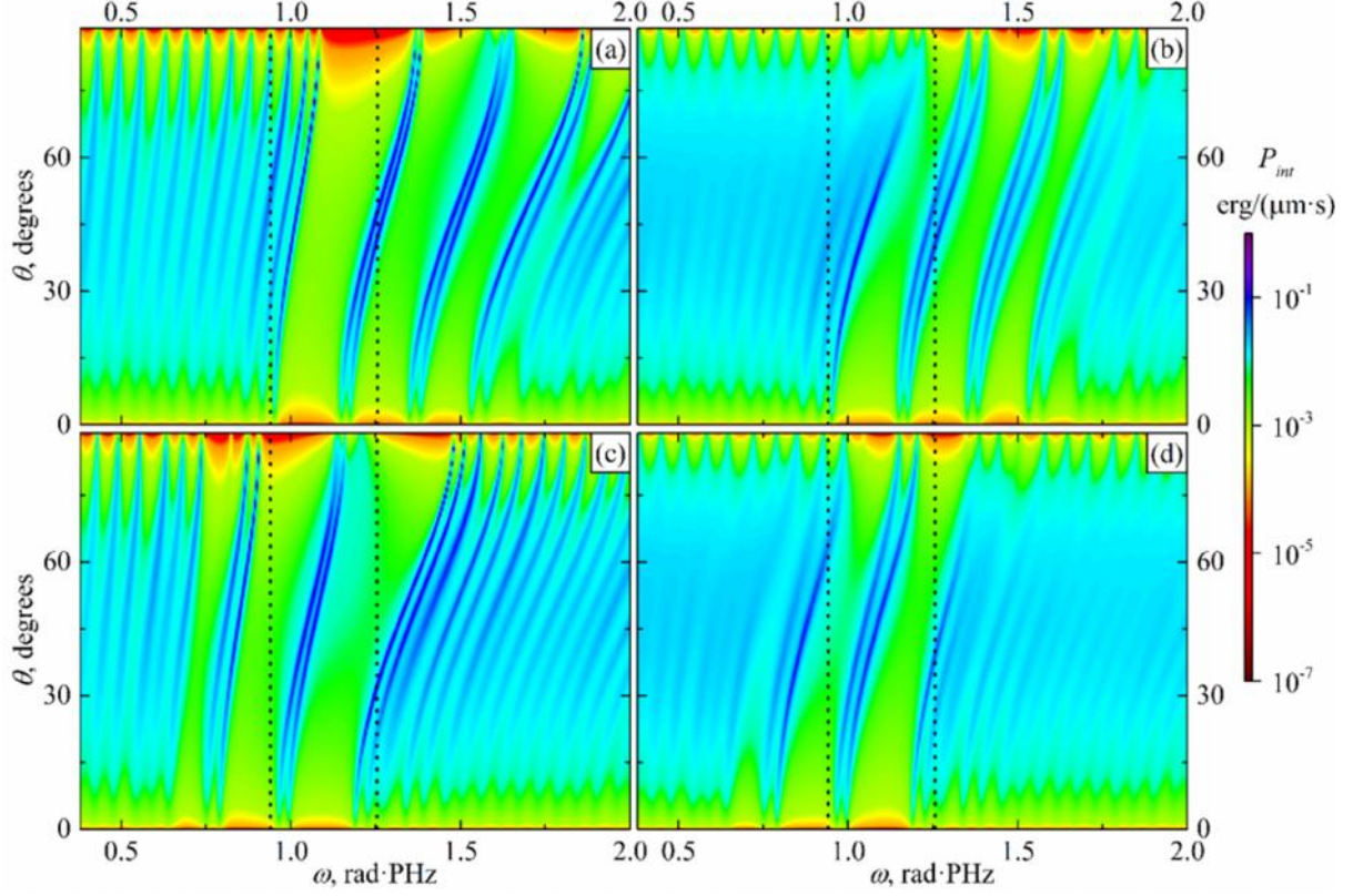
Fig. 5. The integral linear power in the structure [(ST)^3(AZ)^3]^3 as function of the incidence angle \theta_i and frequency \omega for \lambda_{oh} = 1.5 \mu\text{m} , \lambda_{ot} = 2 \mu\text{m} [(a) and (b)] and \lambda_{oh} = 2 \mu\text{m} , \lambda_{ot} = 1.5 \mu\text{m} [(c) and (d)]. The left and right columns show the TE- and TM-modes, respectively.
