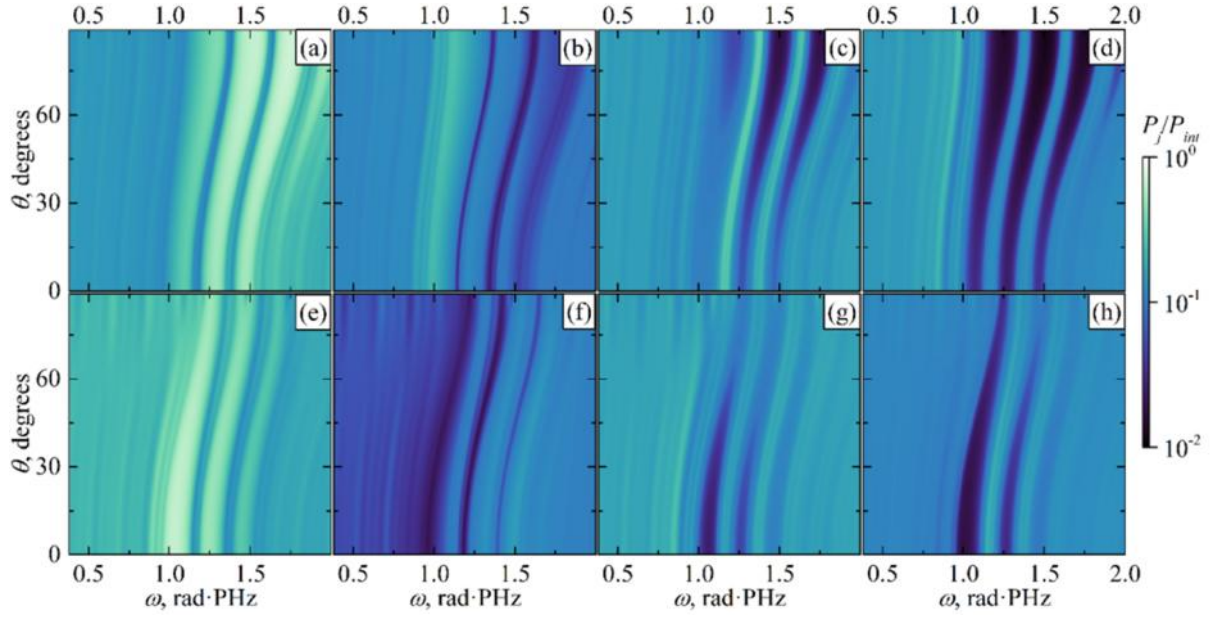
Fig. 6. Reduced partial linear powers P_f/P_{int} in the layers S, T, A, and Z (from the left to the right, the 1 st , the 2 nd , the 3 rd , and the 4 th columns, respectively) in the structure [(ST)^3(AZ)^3]^3 for the TE- and TM- modes (the top and the bottom rows, respectively). The PBG center wavelengths are \lambda_{0h} = 1.5 \mu\text{m} , \lambda_{0r} = 2 \mu\text{m} .
