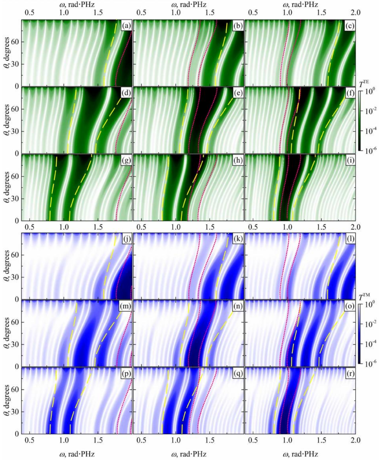
Fig. 3. Transmission spectra T(., \tilde{S}) of the structure [(ST)^3(AZ)^3]^3 for TE- [the top panel (a)-(i)] and TM- [the bottom panel (j)-(r)] modes at various values of \}_{oh} and \}_{ol} . In the top row, \}_{oh} = 1.0 \mu\text{m} ( \tilde{S}_{oh} = 1.885 \text{ rad}\cdot\text{PHz} ), in the middle row, \}_{oh} = 1.5 \mu\text{m} ( \tilde{S}_{oh} = 1.257 \text{ rad}\cdot\text{PHz} ), in the bottom row, \}_{oh} = 2.0 \mu\text{m} ( \tilde{S}_{oh} = 0.942 \text{ rad}\cdot\text{PHz} ); in the left column, \}_{ol} = 1.0 \mu\text{m} , in the middle column, \}_{ol} = 1.5 \mu\text{m} , in the right column, \}_{ol} = 2.0 \mu\text{m} . The yellow dashed and the red dotted lines show the PBG edges of single-periodic PCs formed by the high- and low-optical-contrast subcells (ST)^9 and (AZ)^9 , respectively.
