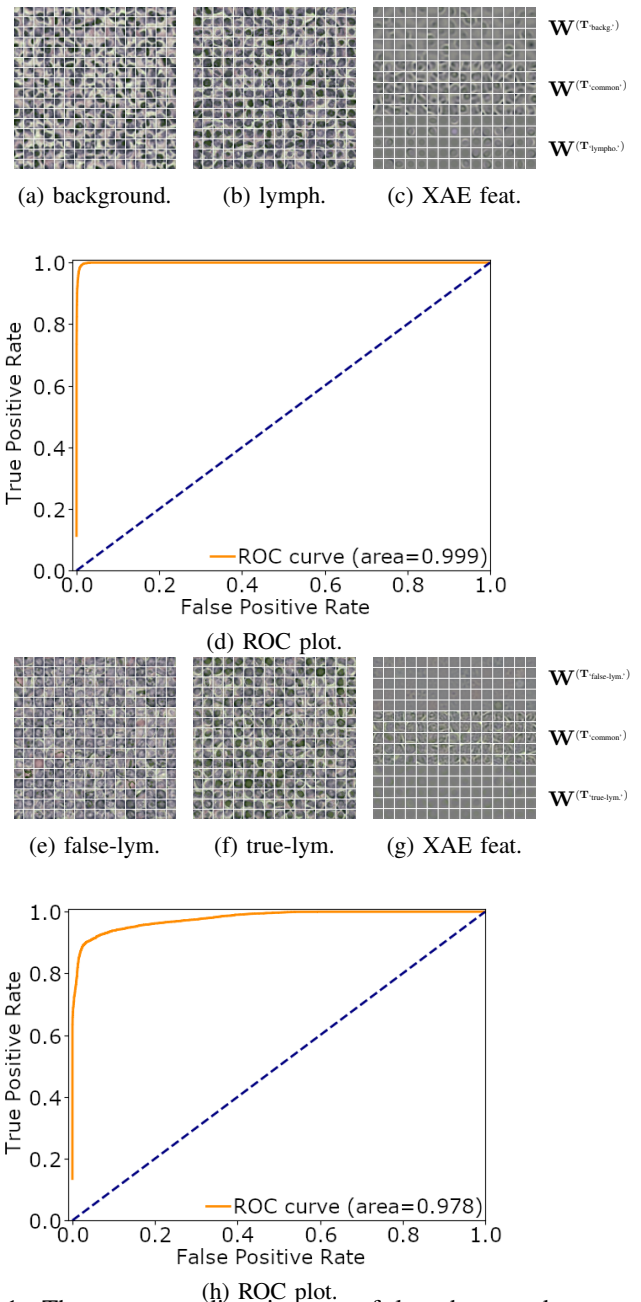
Fig. 1: The corresponding images of lymphocyte detection/classification and the corresponding ROC plots: (a)-(d) lymphocyte detection; (e)-(h) lymphocyte classification.
