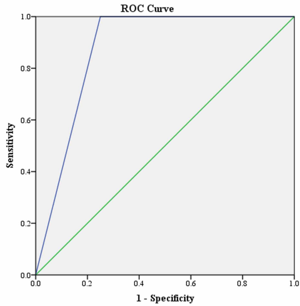
Figure 10: ROC curve
