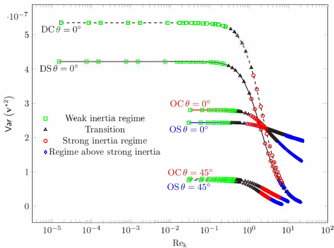
FIG. 10. Variance of the fluid kinetic energy, \text{Var}(\mathbf{v}^{*2}) , versus the Reynolds number \text{Re}_k for the model porous structures of Fig. 1 (OS, OC, DS, and DC) and two different orientations of \nabla\langle p^*\rangle^\beta : \theta = 0^\circ ( \nabla\langle p^*\rangle^\beta = \hat{\mathbf{e}}_x ) and \theta = 45^\circ [ \nabla\langle p^*\rangle^\beta = (\hat{\mathbf{e}}_x + \hat{\mathbf{e}}_y)/\sqrt{2} ]. Identification of flow regimes from data in Table I. Porosity \epsilon = 75\% .
