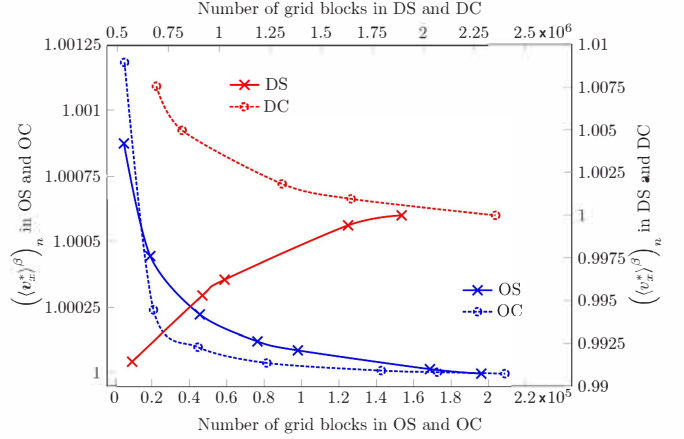
FIG. 3. Normalized intrinsic average of the x component of the velocity, ((v_x^*)^\beta)_n , versus the number of grid blocks. Model porous structures of Fig. 1. Normalization with respect to (v_x^*)^\beta obtained with the finest mesh. OS, \text{Re}^* = 17\,500 ( \text{Re}_k = 23.41 ); OC, \text{Re}^* = 17\,500 ( \text{Re}_k = 21.09 ); DS, \text{Re}^* = 30\,000 ( \text{Re}_k = 18.58 ); DC, \text{Re}^* = 30\,000 ( \text{Re}_k = 19.87 ); \epsilon = 75\% ; \nabla \langle p^* \rangle^\beta = \hat{\mathbf{e}}_x .
