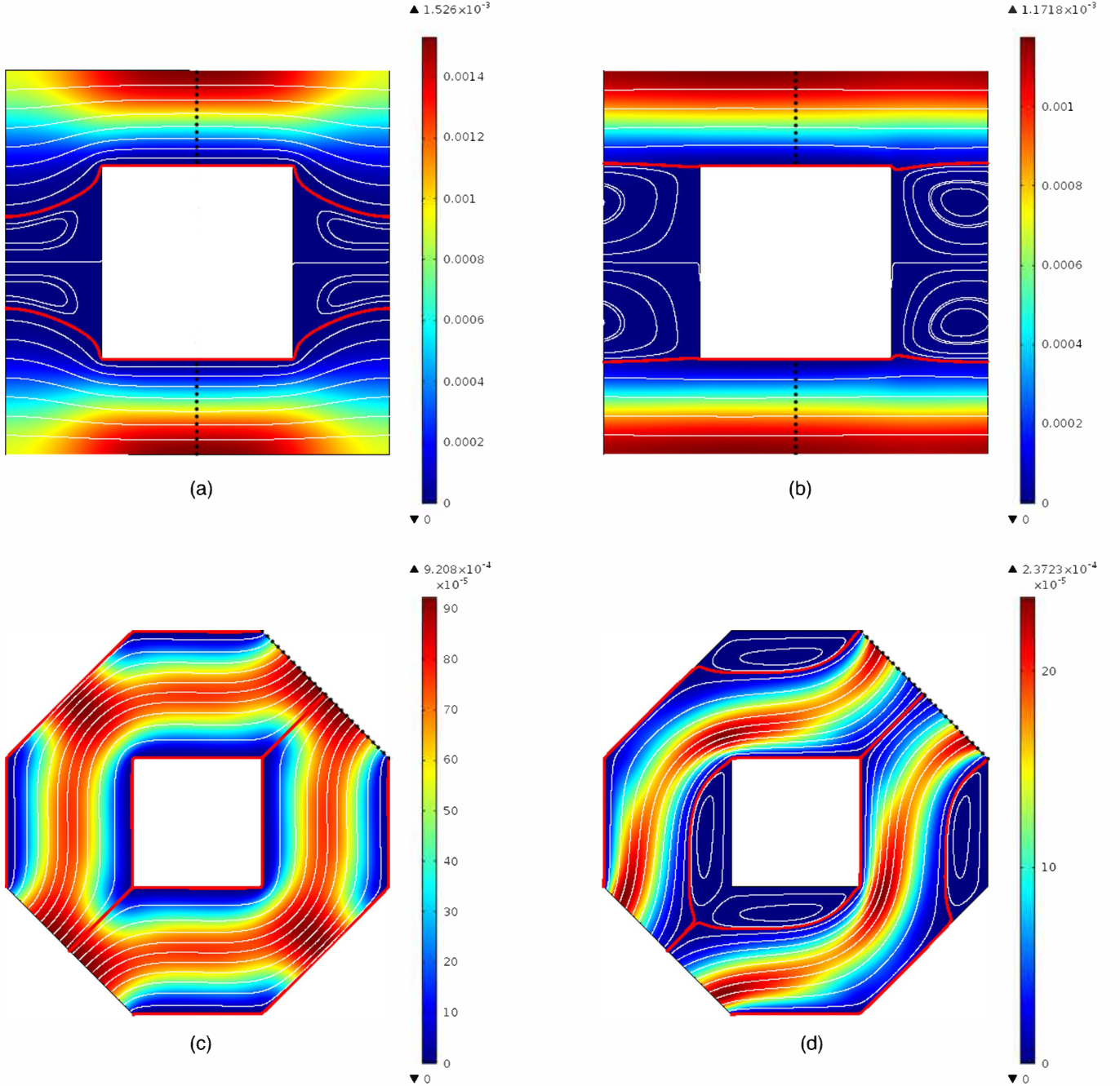
FIG. 5. Fluid kinetic energy color map, \mathbf{v}^{*2} , and steady flow streamlines in the OS of Fig. 1. The thick red streamlines delimit recirculation zones. The dotted line represents an arbitrary cross section S \perp \nabla \langle p^* \rangle^\beta . (a) \text{Re}_k = 0 , (b) \text{Re}_k = 23.41 , (c) \text{Re}_k = 0 , (d) \text{Re}_k = 6.76 . (a and b) \theta = 0^\circ ( \nabla \langle p^* \rangle^\beta = \hat{\mathbf{e}}_x ). (c and d), \theta = 45^\circ [ \nabla \langle p^* \rangle^\beta = (\hat{\mathbf{e}}_x + \hat{\mathbf{e}}_y)/\sqrt{2} ]. Porosity \epsilon = 75\% .
