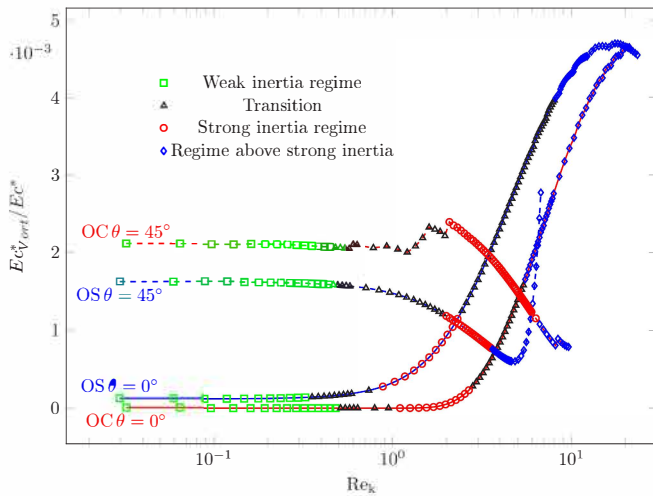
FIG. 7. Ratio between the fluid kinetic energy in the vortices and the total fluid kinetic energy, Ec_{\text{vort}}^*/Ec^* , versus the Reynolds number \text{Re}_k . Ordered model porous structures OS and OC of Fig. 1. Two different orientations of the macroscopic pressure gradient, \theta = 0^\circ and \theta = 45^\circ . Identification of flow regimes from data in Table I. Porosity \epsilon = 75\% .
