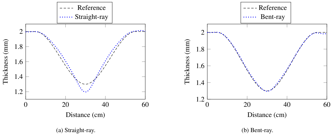
Fig. 10. Ray-tomography with refraction only (defect 1).
