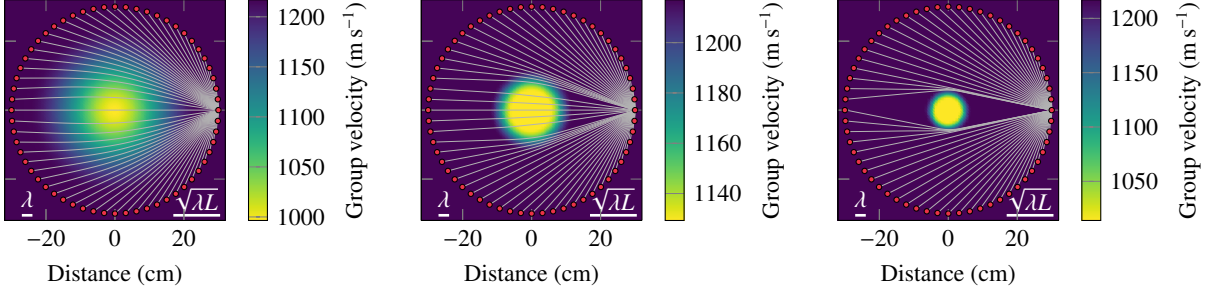
(a) Defect 1 - Only refraction phenomenon. e_{\text{def}} = 0.7 mm, r_{\text{bot}} = 0 cm and l_{\text{trans}} = 25 cm (see Fig. 8 and Eq. (13) for the definitions).
