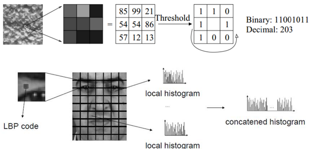
Figure 21. Example of facial local binary pattern (LBP) calculation.
