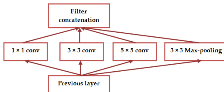
Figure 25. GoogleNet architecture.
