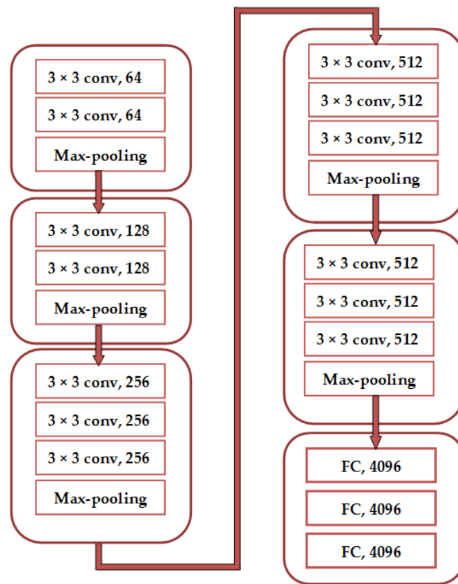
Figure 24. VGGNet architecture.
