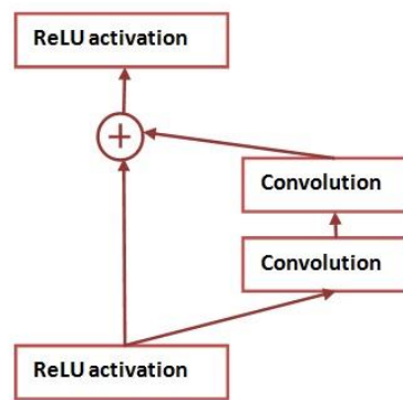
Figure 26. ResNet architecture.
