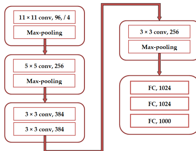
Figure 23. AlexNet architecture. FC (fully connected layer): fully connected layers. conv: convolution.
