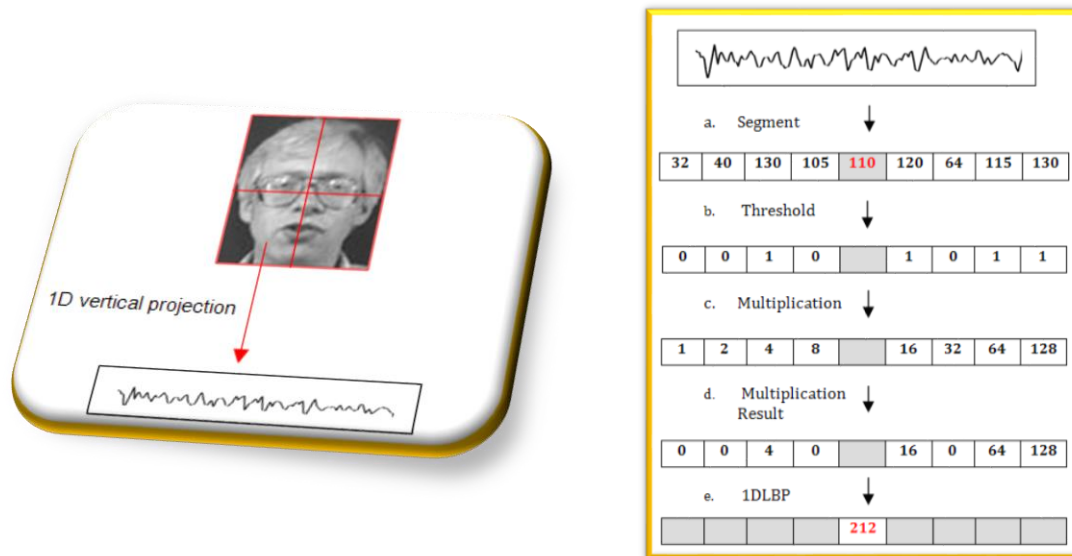
Figure 22. Example of one-dimensional local binary pattern (1DLBP) facial calculation.
