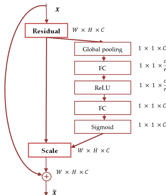
Figure 27. SENet architecture. X : the input. W \times H : spatial dimensions. C : channel descriptor. r : reduction ratio. FC: fully connected layers. \tilde{X} : the output.
