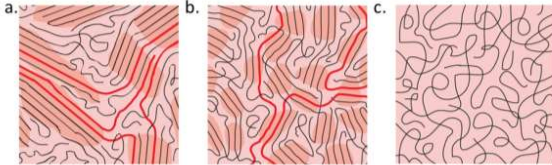
Figure 1. Schematic structure of polymers with different disorder levels. (a) Very ordered, (b) disordered aggregates and (c) completely disordered. Depending on the density of the polymer, long chains (highlighted in red) can connect ordered regions (darker orange ones) without significant loss of the conjugation length. [28]. Copyright 2013, Springer Nature.
