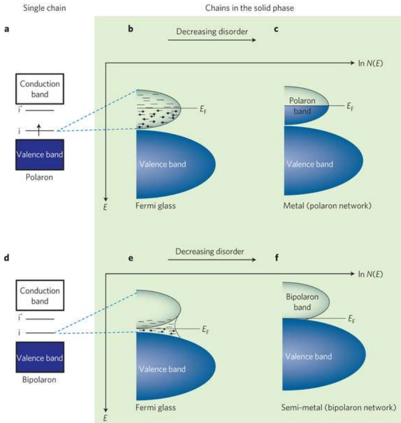
Figure 32. Representation of the electronic structure in PEDOT materials and in conducting polymers in general. a–c, If the majority charge carriers are polarons: (a) a polymer chain with one polaron, (b) the logarithm of the density of states (DOS) \ln N(E) disordered material (c) as well as for a more ordered (metallic) system. In the latter case, the Fermi level lies in a delocalized polaron band while it was surrounded with localized states in the former case. d–f, If the majority charge carriers are bipolarons: (d) a polymer chain with one bipolaron, (e) \ln N(E) for an disordered bipolaronic polymer solid, (f) as well as for a more ordered (semi-metallic) solid. The Fermi level lies between the valence band and the empty bipolaron band in the latter case.[163] Copyright 2013, Springer Nature.
