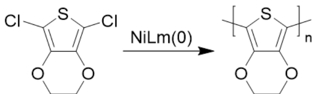
Figure 8. Nickel based polycondensation for neutral PEDOT synthesis. [73]
