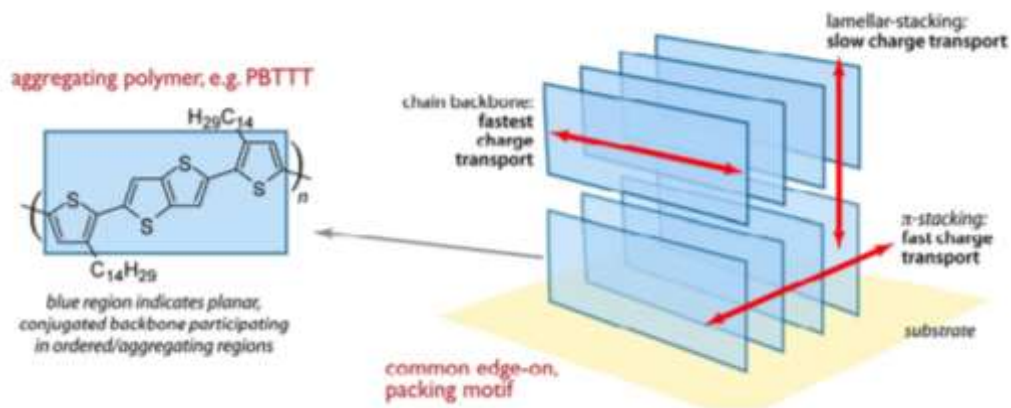
Figure 2. Fast, moderate and slow transport along the chain backbone, the \pi - \pi stacking and the lamellar stacking respectively in conducting polymers.[28]. Copyright 2013, Springer Nature.
