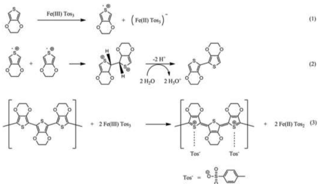
Figure 9. Proposed mechanism for the synthesis of PEDOT:Tos as reproduced from Mueller and coworkers' work.[79] Copyright 2012, Elsevier Ltd. (copyright review from Elsevier requested).
