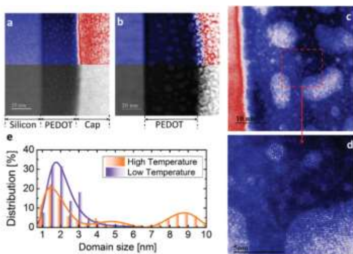
Figure 26. The HAADF STEM image of cross sections of the interfaces of grafted PEDOT films grown at (a) 100 °C and (b) 200 °C. The top halves of both images are color-enhanced to clearly elucidate the crystalline domains surrounded by an amorphous matrix. High-resolution images for the film synthesized at 200 °C are shown in (c) and enlarged in (d), providing a direct evidence on the well-organized large crystallites. (e) Histogram of statistical domain size distribution obtained from images (a) and (b), showing the broader distribution and larger crystallite size for the film grown at high temperature (200 °C).[99]
