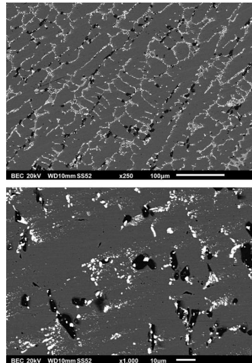
Figure 10. The microstructure of the Th alloy after 50h at 1250°C (SEM/BSE micrograph)
