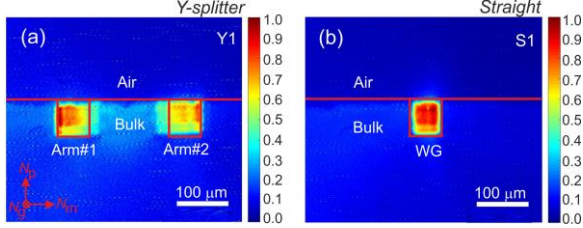
Fig. 9. Near-field pump mode profiles for the (a) Y-branch (Y1) and (b) straight (S1) WGs fs-DLW in Tm:KLuW. Red lines – air/crystal interface and WG cladding drawn as a guide for the reader. The pump polarization ( E \parallel N_m ) is horizontal. P_{inc} = 0.5 W.
