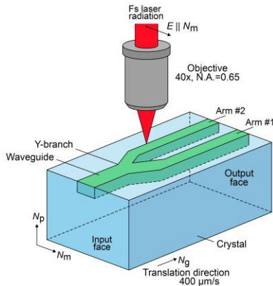
Fig. 1. Scheme of femtosecond direct laser writing of Y-branch waveguides in monoclinic \text{Tm:KLuW} crystals: N_p , N_m and N_g – optical indicatrix axes.
