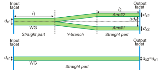
Fig. 2. Scheme of Y-branch and straight WGs exhibiting rectangular cross-sections (top-view).
