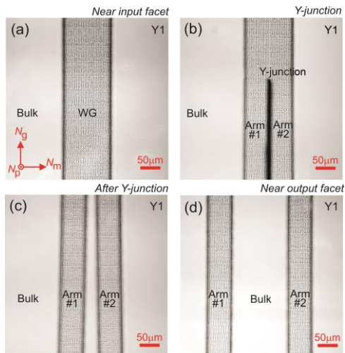
Fig. 4. Top-view confocal laser microscope images of (a-d) various parts of the Y-branch splitter Y1 fabricated by fs-DLW in Tm:KLuW. Transmission mode, polarized light ( P \parallel N_g ), \lambda = 405 nm.
