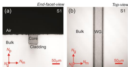
Fig. 6. (a) End-facet-view and (b) top-view confocal laser microscope images of the straight WG S1 exhibiting a rectangular cross-section fabricated by fs-DLW in Tm:KLuW. Transmission mode, polarized light: (a) P \parallel N_p and (b) P \parallel N_g , \lambda = 405 nm.
