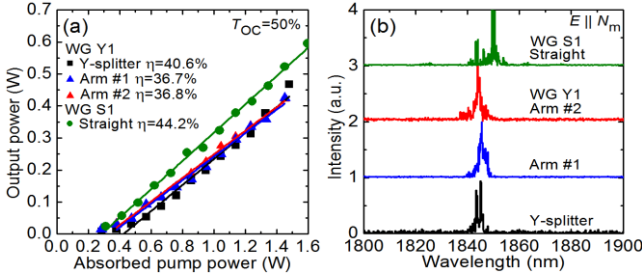
Fig. 12. (a) Input-output dependences and (b) typical laser emission spectra measured at maximum P_{\text{abs}} for Y-branch and straight WGs (Y1 and S1) fabricated by fs-DLW in Tm:KLuW operated under different regimes, \eta – slope efficiency. The laser polarization is \mathbf{E} \parallel N_m .
