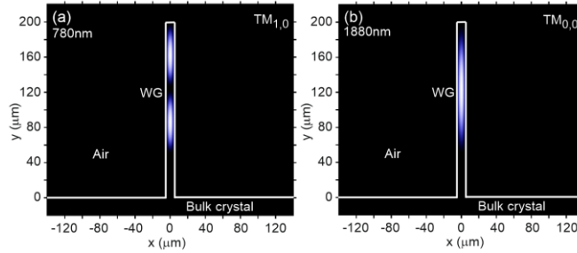
Fig. 5. Simulated 2D intensity mode profiles in the 10 \mu\text{m} wide WG at the light wavelength of (a) 780 nm (pump, TM 1,0 mode) and (b) 1880 nm (laser, TM 0,0 mode). The light polarization is vertical. The refractive index increase in the guide \Delta n is \sim 2.5 \times 10^{-3} , n_e = 1.4728 (780 nm) and n_e = 1.4652 (1880 nm).
