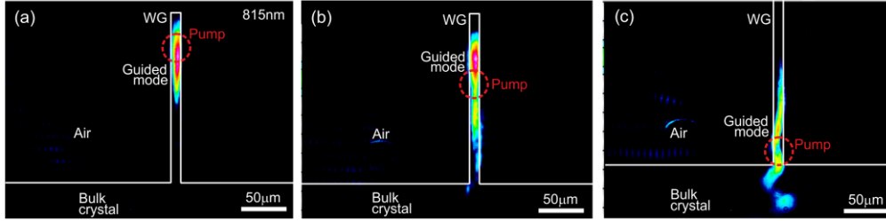
Fig. 4. 2D intensity profiles of the guided pump mode at the output WG facet: focusing of the pump beam in (a) the top part, (b) the medium part and (c) bottom part of the 10 \mu\text{m} wide WG. White lines showing the crystal surface are drawn as guides for eyes. Red dashed circles indicate the position of the pump beam at the input facet. \lambda_p = 815 nm. The laser polarization ( \pi ) is vertical.
