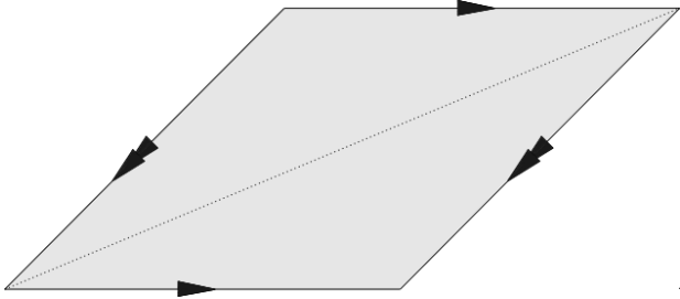
Figure 3: The Möbius strip as a quotient.
