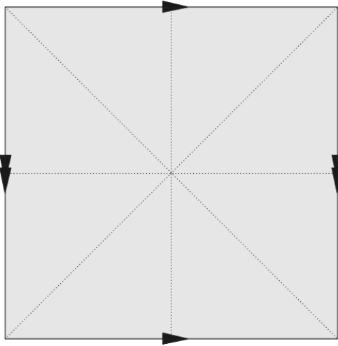
Figure 6: A 45^\circ triangle rectangle as a quotient.
