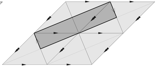
Figure 4: The Möbius strip.
