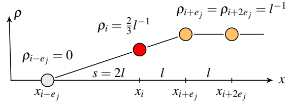
Figure 6. Left boundary of the system (61) with control (70). Agent i is on the boundary, the position of the "ghost agent" i - e_j is chosen such that \rho linearly goes to zero at x_{i-e_j} .
