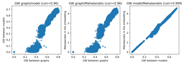
Figure 4. Plot of the pairwise distances in D_1 and their Pearson correlation coefficients. GW distance between graphs versus its counterpart between the embedded graphs (left). GW distance between graphs versus Mahalanobis distance between the embeddings (middle). GW distance between the embedded graphs versus Mahalanobis between the corresponding embeddings (right).
