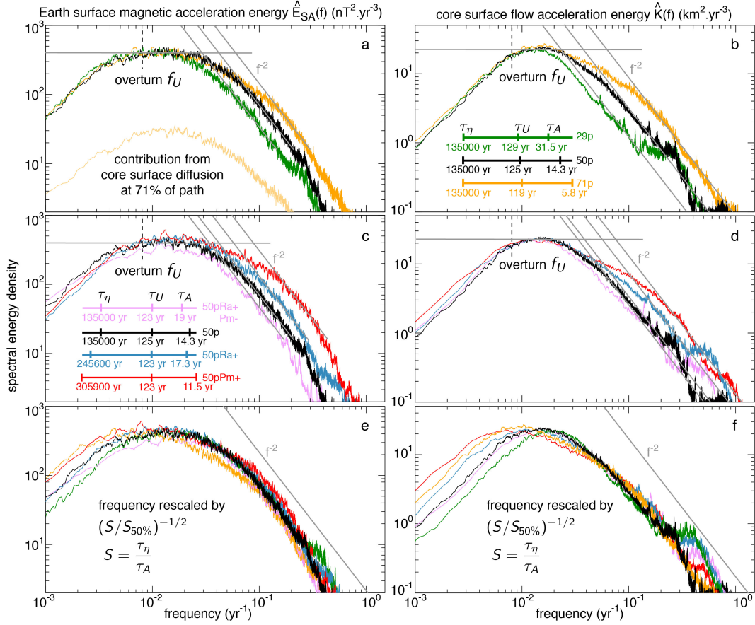
Fig. 5. Frequency domain spectral density \hat{E}_{SA}(f) of the magnetic acceleration energy at Earth's surface (a,c,e), and \hat{K}(f) of the flow acceleration energy at the core surface (b,d,f), for models taken along (a,b) and across (c,d) the parameter space path. a,b: spectra of the 29 percent, 50 percent and 71 percent of path models, plotted together in a. with the additional contribution of core surface magnetic diffusion in the 71p model. b,d: spectra of the 50 percent of path, 50pRa+Pm-, 50pRa+ and 50pPm+ models. In a-d the dashed vertical line marks the overturn frequency f_U = 1/\tau_U . Flat and slanted grey lines respectively mark the power-laws f^0 and f^{-2} , the crossing of which defines the cut-off frequency f_c . The relative positions and numerical values of the time scales \tau_\eta , \tau_U and \tau_A are also recalled. e,f: respective compounds of a,c and b,d, with frequency axis rescaled for each model by (S/S_{50\%})^{-1/2} , where S = \tau_\eta/\tau_A and S_{50\%} is the Lundquist number of the Midpath model.
