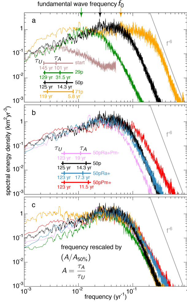
Fig. 7. Frequency domain spectral density \hat{K}^{ZS}(f) of the core surface azimuthal, equator-symmetric and axisymmetric acceleration energy for models taken (a) along and (b) across the parameter space path. a: spectra of the start, 29 percent, 50 percent and 71 percent of path models. b: spectra of the 50 percent of path, 50pRa+Pm-, 50pRa+ and 50pPm+ models. The numerical values of the time scales \tau_U and \tau_A are also recalled in a,b. In a., the arrows locate the frequency of the fundamental Alfvén wave f = (\sqrt{3}r_o\tau_A)^{-1} for models along the path, and the slanted grey line marks the power law f^{-6} . c: compound of a.,b., with frequency axis rescaled for each model by A/A_{50\%} , where A = \tau_A/\tau_U and A_{50\%} is the Alfvén number of the Midpath model.
