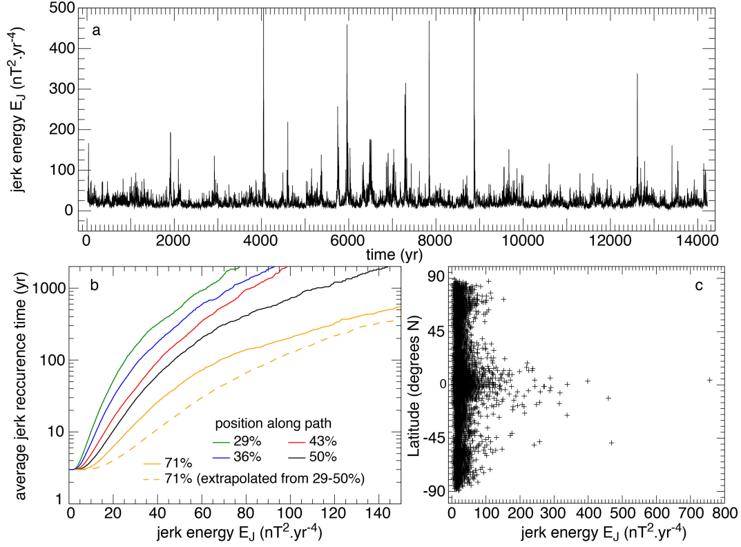
Fig. 4. a: Time series of the Earth surface jerk energy E_J (see section 2.5). b: Distribution of jerk energy as a function of the jerk recurrence time, for models previously computed in the range 29 percent to 50 percent of the parameter space path (Aubert & Finlay, 2019) and the 71p model. Shown in dashed line is the expected distribution at 71 percent of the path from an extrapolation E_J \sim \epsilon^{-0.19} previously obtained from the behaviours between 29 and 50 percent of the path (Aubert & Finlay, 2019). c: Distribution of jerk energy in the 71p model (sampled each year) as a function of the latitude of the amplitude maxima observed in the radial magnetic acceleration at the core surface. Jerk statistics in b,c are computed in the time window [4200 yr, 14200 yr] where the spatio-temporal resolution of the computation is optimal (see coloured bands under Fig. 3b). This interval also avoids two spurious acceleration pulses near times 1130 and 4180 years, corresponding to resolution changes.
