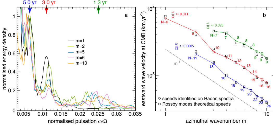
Fig. 10. a: Frequency-domain energy density profiles of \dot{u}_\varphi at the equator in a 130-year sequence of the 71p model. The acceleration signal is broken down into contributions from distinct azimuthal mode numbers m and the energy is normalised relative to the peak at \omega/\Omega \approx 0.0065 . Also reported at the top of the graph are the periods corresponding to each of the three identified peaks (located by colored arrows). b: Eastward propagation velocities (circles) identified on Radon-transformed time-longitude diagrams of equatorial azimuthal flow acceleration (following the procedure described in Finlay, 2005), represented as a function of the mode number m at each of the three normalised pulsations \omega/\Omega \approx 0.0065, 0.011, 0.025 corresponding to the peaks in panel a (see arrows of same color). Also reported as functions of m are the closest matching phase velocities c = \omega r_o/m (squares) obtained by adjusting the radial complexity number N in equation (18). The grey line represents a m^{-1} law.
