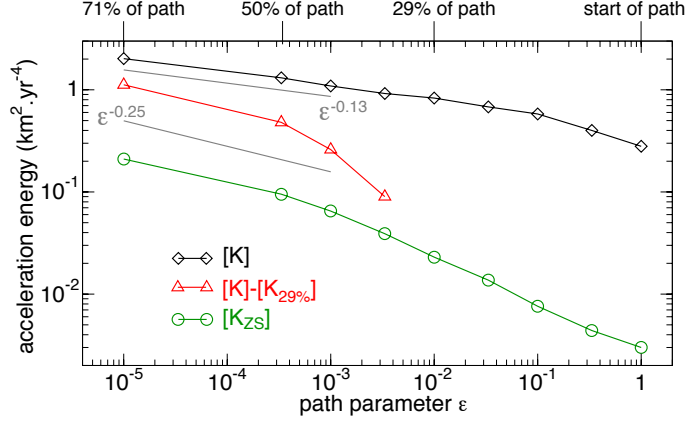
Fig. 11. a: Evolution with the path parameter \epsilon of the time-averaged, total core surface flow acceleration energy [K] up to spherical harmonic degree 30, plotted together with two diagnostics of the evolution of wave energy along the path (Earth's core conditions are towards the left of the graph). The energy of axisymmetric torsional waves is represented by the axisymmetric, azimuthal and equator-symmetric part [K^{ZS}] , and the energy of non-axisymmetric waves is represented by the difference [K] - [K_{29\%}] of [K] to its value at 29 percent of the path. The grey lines mark the \epsilon^{0.13} and \epsilon^{0.25} power-law behaviours.
