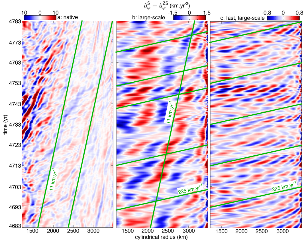
Fig. 9. Time-cylindrical radius diagrams of the non-axisymmetric, equator-symmetric core surface azimuthal flow acceleration \dot{u}_\varphi^S - \dot{u}_\varphi^{ZS} at longitude 112.5^\circ\text{E} (located by arrows in Fig. 8c,d) in the 71p model, presented at (a) native spatial and temporal resolution, (b) large-scale (spherical harmonic degree up to 30), and (c) large-scale for the fast component obtained after removal of a 5-year running average in time. The sets of slanted green lines denote advection at the one-dimensional convective velocity D/\sqrt{3}\tau_U = 11 \text{ km/yr} , and propagation at the one-dimensional Alfvén wave velocity D/\sqrt{3}\tau_A = 225 \text{ km/yr} .
