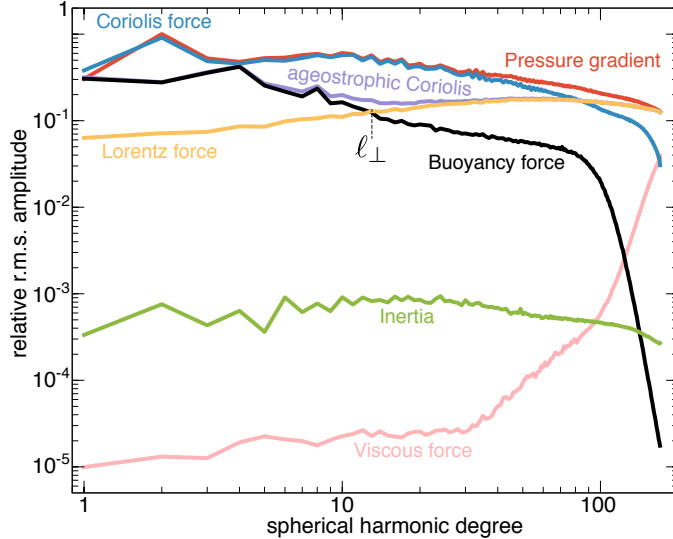
Fig. 1. Root-mean-squared amplitude of the forces in a snapshot of the 71p model, presented as functions of the spherical harmonic degree \ell (see section 2.3). All forces are normalised respectively to the maximum reached by the pressure gradient. The snapshot was taken from the later part of the run where \ell_{\max} = 170 and q_h = 1.09 (see Fig. 3).
