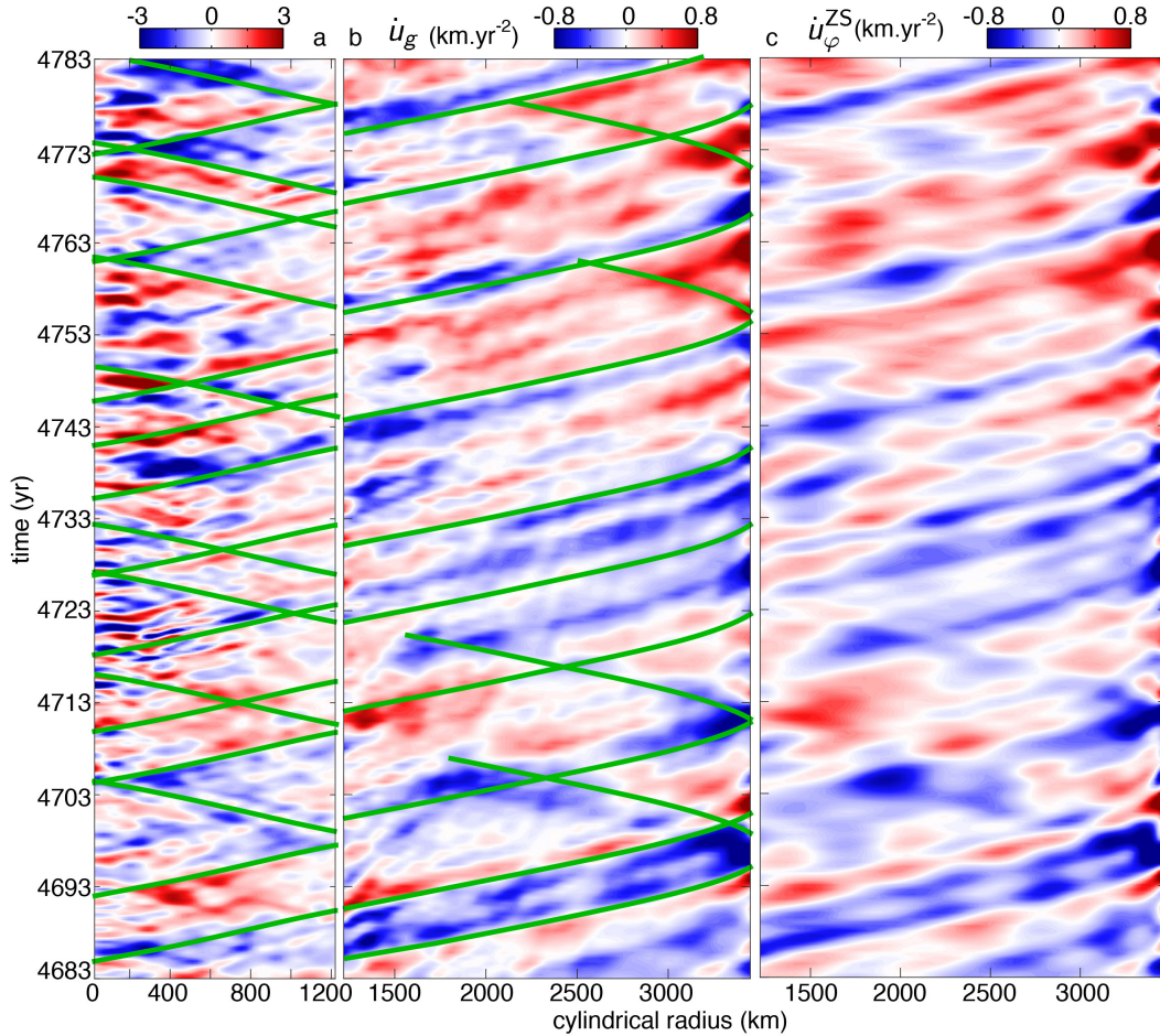
Fig. 6. Time-cylindrical radius diagrams of the geostrophic flow acceleration \dot{u}_g (equation 9) sampling the interior of the fluid in the Northern part of the tangent cylinder (a), and the region outside the tangent cylinder (b), at native resolution in the 71p model. c: time-cylindrical radius diagram obtained at the core surface and outside the tangent cylinder by representing the equator-symmetric, axisymmetric azimuthal flow acceleration \dot{u}_\varphi^{ZS} up to spherical harmonic degree 30. Note the larger extremes of the color map in a. relatively to b,c. Green curves in a.,b. correspond to outwards and inwards ray-tracing theoretical propagation tracks at the column-averaged Alfvén speed c_A(s, t) (equation 10).
