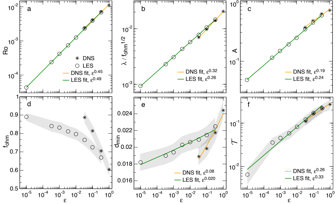
Fig. 2. Evolution of the Rossby number Ro (a), Lehnert number \lambda (b), Alfvén number A (c), Ohmic fraction f_{\text{ohm}} (d), magnetic dissipation length scale d_{\text{min}} (e) and Taylor constraint enforcement level \mathcal{T} (f) along the parameter space path, as functions of the path parameter \epsilon (Earth’s core conditions are towards the left of the graphs). Shown are results from hyperdiffusive solutions along the path (LES or large-eddy-simulations) up to 71 percent of the path ( \epsilon = 10^{-5} ), and the direct numerical simulations (DNS) up to 21 percent of the path ( \epsilon = 3.33 \cdot 10^{-2} ). See Tables 2a and 3 for data between 29 and 71 percent of the path, and Aubert et al. (2017); Aubert (2019) for other numerical values. Green and orange lines respectively show the results of least-squares power-law fits to the LES and DNS data, which closely adhere to the theories of Aubert et al. (2017); Davidson (2013), respectively. Shaded grey areas represent the \pm 1 standard deviation, where applicable.
