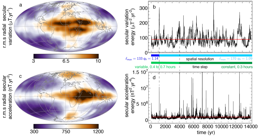
Fig. 3. Magnetic variation and acceleration properties of the 71p model. a,c: Hammer projections of the time-averaged, root-mean squared radial magnetic variation \mathbf{\hat{B}} \cdot \mathbf{e}_r (a) and acceleration \mathbf{\hat{B}} \cdot \mathbf{e}_r (c) at the core surface, from magnetic field output up to spherical harmonic degree 13. b,d: Time series of the magnetic variation and acceleration energies E_{SV} (b) and E_{SA} (d) at the core surface. Red lines in (b,d) mark the time-averaged values [E_{SV}] and [E_{SA}] . The blue and green bands between (b) and (d) locate the notable events related to spatial and temporal resolution changes in the model computation.
