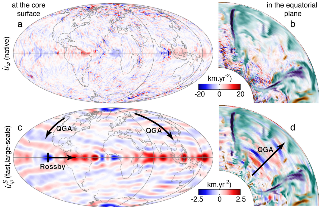
Fig. 8. State of the 71p model at time 4749.8 yr of the simulation. Core surface Hammer projections (a,c) and partial equatorial plane views (b,d) of the azimuthal flow acceleration. In a,b, the total azimuthal acceleration \dot{u}_\varphi is presented at native spatial and temporal resolution. In c,d, the fast and large-scale component of the equator-symmetric azimuthal acceleration \dot{u}_\varphi^S is presented. The fast component is obtained after removal of a 5-year running average. The large-scale component is obtained in c. by truncation after spherical harmonic degree 30, and in d. by lateral truncation after azimuthal wavenumber 30 and application of a running average of thickness 40 km in the radial direction. For clarity also, accelerations larger than 4 \text{ km.yr}^{-2} are not represented in d. The partial equatorial views in b,d, are taken between the grey meridians delineated in a,c. In these equatorial views also, the density anomaly (green-brown, maximal values \pm 0.5 \cdot 10^{-4} \text{ kg/m}^3 ) and radial magnetic field (orange-purple, maximal values \pm 9.5 \text{ mT} ) are represented in a selectively transparent manner. Black arrows in c,d, denote the propagation direction of quasi-geostrophic Alfvén (QGA) and Rossby waves. The QGA wave arrow in d. also marks the longitude selected for analysis in Fig. 9.
