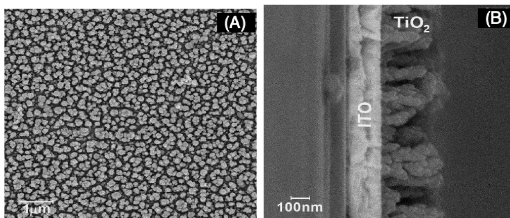
Figure 2. Scanning electron microscopy (SEM) micrographs of indium-doped tin oxide (ITO) | TiO 2 after 300 s electrolysis time (A) top view and (B) cross section.
