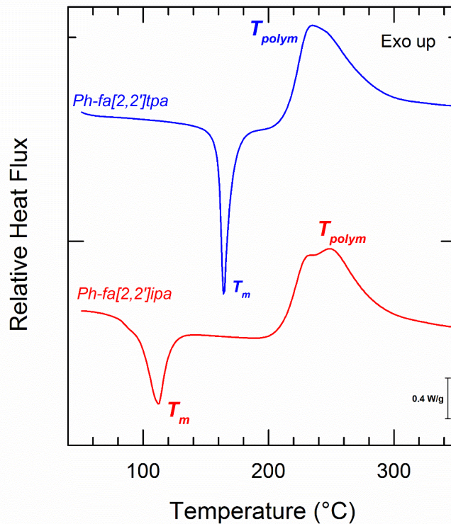
Figure 2 -- DSC of Ph-fa[2,2']ipa and Ph-fa[2,2']tpa at 10\text{ }^{\circ}\text{C}\cdot\text{min}^{-1}
