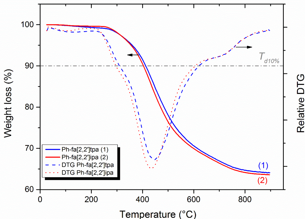
Figure 6 - TGA of cured materials under nitrogen atmosphere
