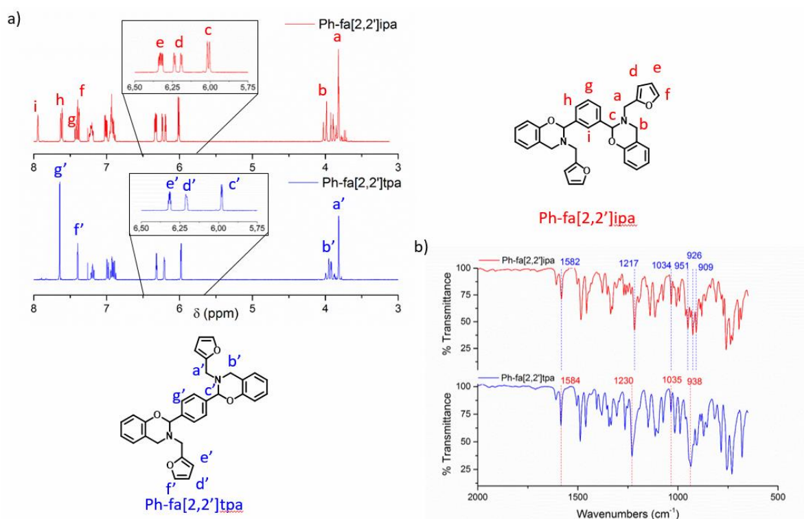
Figure 1 - a) NMR 1H spectra and ; b) FT-IR spectra of both monomers Ph-fa[2,2']ipa and Ph-fa[2,2']tpa
