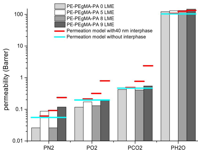
Figure 10. Permeability values for 25/50/25 wt % 0, 5, 8 and 9 LME PE/PEgMA/PA6 with serial model including interphase limits.
