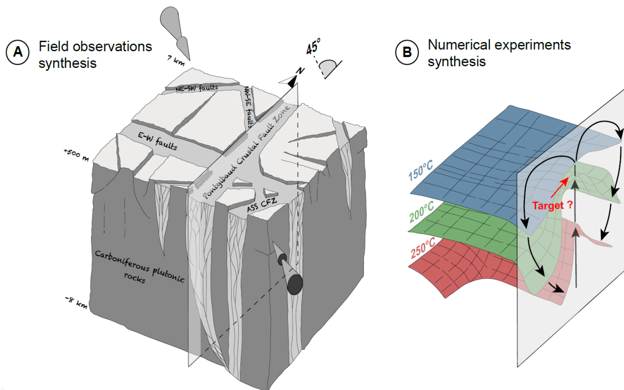
Figure 5: [A] Synthesis of field observations and numerical experiments. The Pontigbaud CFZ is a large deformation zone whose geophysical data (Ars et al., 2019) show deep rooting. [B] The results of the numerical experiments and the comparison with the geothermal gradient and heat flow show that a blob-like fluid circulation would be effective within the Pontigbaud CFZ.
