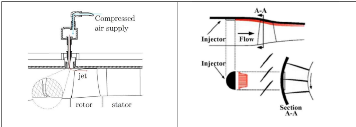
Figure 3. Two examples of tip blowing experiments in axial compressor, from [3] (left) and [8] (right).
