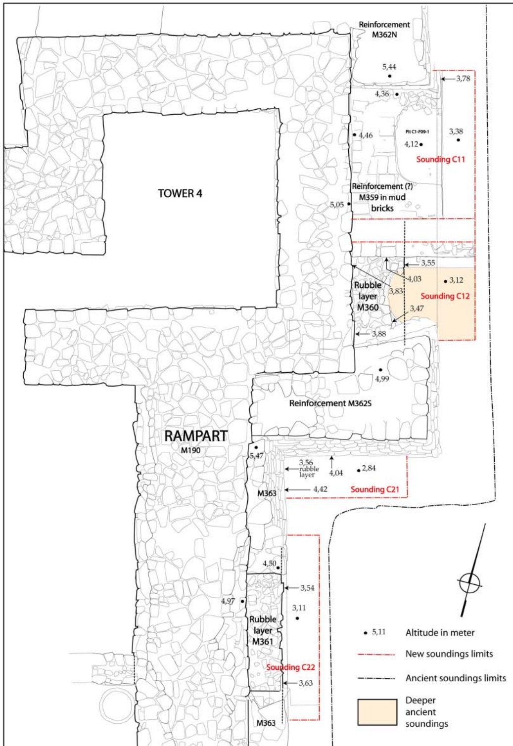
C1 AND C2 SECTORS. E. Laroze, dec. 2009, after O. Callot. Completed by M. Gelin.
