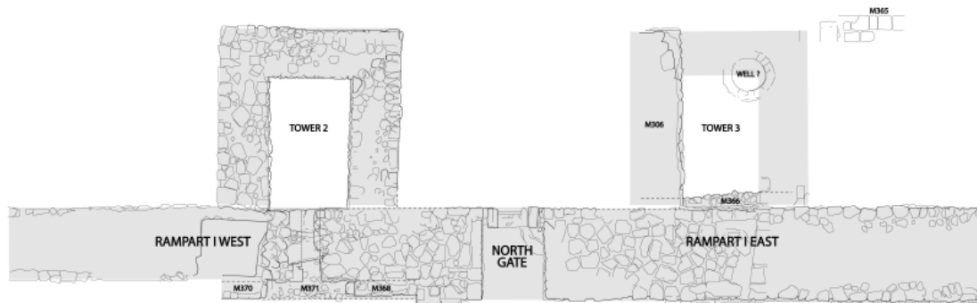
Restitution of the supposed first gate with the two towers and the probable previous outside constructions.
