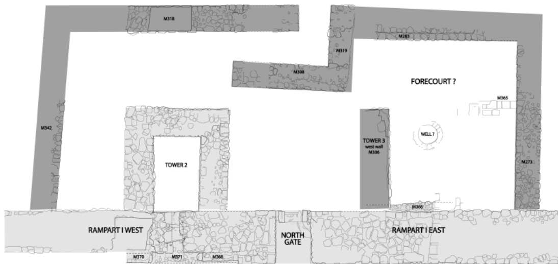
Restitution of the first gate with the later bent-axis walls (chicane) and the probable previous outside constructions.
