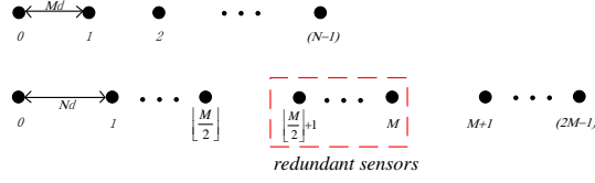
Figure 1: Conventional coprime array.
