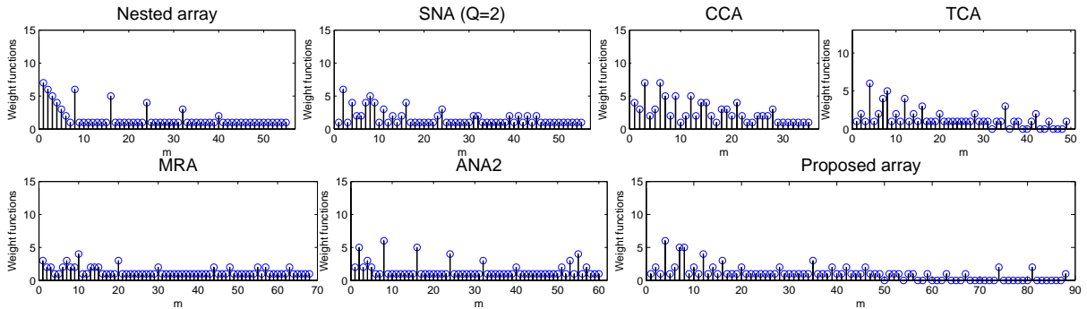
Figure 7: Weight function of seven different arrays.
