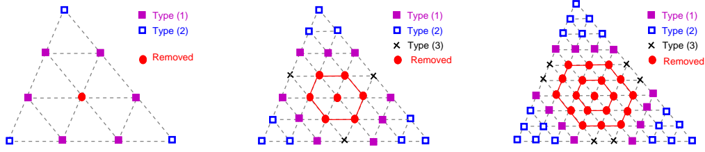
Fig. 1.3 Domain points of the Bernstein polynomials used in the CTS basis, left: r = 1, d = 3 , middle: r = 2, d = 6 , right: r = 3, d = 9 . “Removed” means that the respective Bernstein polynomials are of none of the Types (1), (2) or (3).
