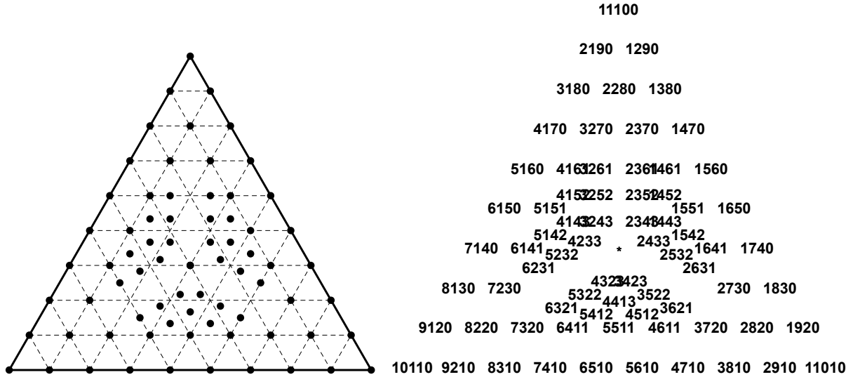
Fig. 1.7 Simplex splines domain points on the right, with their positions on the left. S_{3324}^9, S_{3234}^9, S_{2334}^9 have the same domain point (1/3, 1/3, 1/3) as indicated by a *
