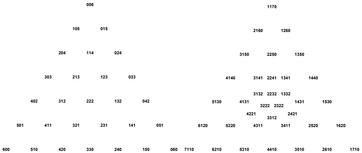
Fig. 1.4 Bernstein domain points on the left, Simplex splines domain points on the right.
