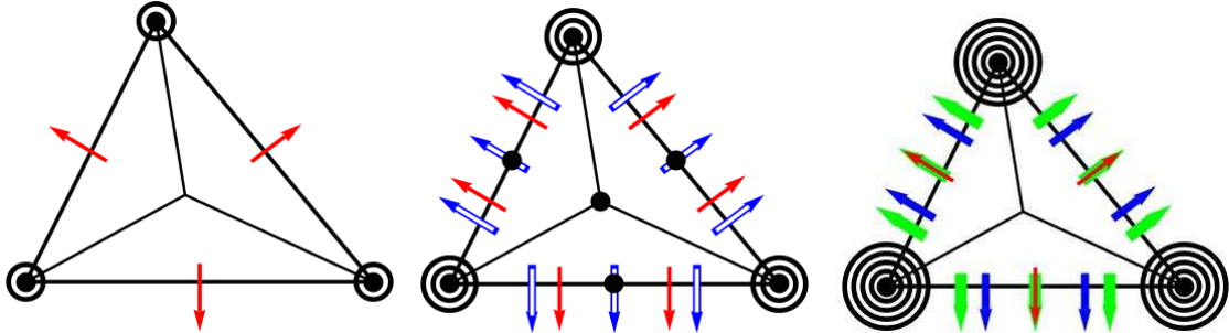
Fig. 1.2 The degrees of freedom cs_{3r}^r for C^1 , C^2 and C^3 . For the order of a cross boundary derivative D_{n_i}^\alpha we use a dot for \alpha = 0 , and colors red, blue and green for \alpha = 1, 2, 3 .
