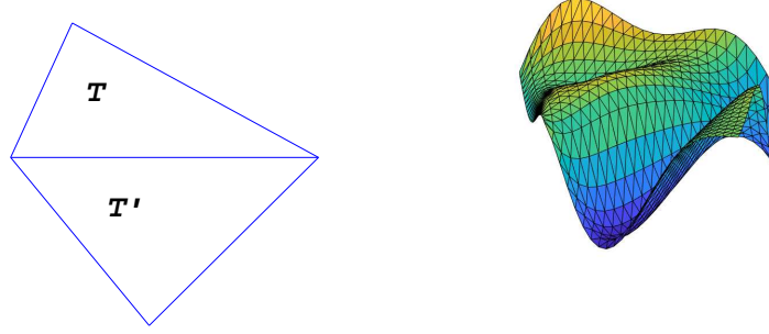
Fig. 1.6 A C^2 surface on two triangles
