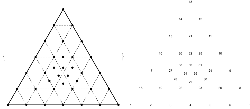
Fig. 1.5 The position, left, and ordering of the domainpoints and corresponding basis functions in Figure 1.4, right.
