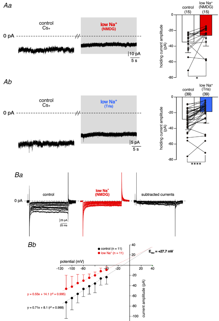
Figure 10. I_{\text{Nab}} is not blocked by \text{Cs}^+ A , effects of low \text{Na}^+ saline on the holding current of CCs patched with a pipette solution containing 140 mM \text{CsCl} and clamped at -50 mV. Bath-applied low \text{Na}^+ salines (NMDG- ( Aa ) or a Tris- ( Ab ) replaced) decreased the holding current value, indicating that I_{\text{Nab}} is not inhibited by \text{Cs}^+ . Mean holding current amplitude: -35.3 \pm 13.4 pA versus -26.8 \pm 13.5 pA, in control and NMDG-containing saline, respectively, n = 15 cells, P < 0.05 ( = 0.0256 ), Wilcoxon matched-pairs signed-rank test and -28.9 \pm 13.5 pA versus -19.3 \pm 14.6 pA, in control and Tris-containing saline, respectively, n = 39 cells, P < 0.0001 , Wilcoxon matched-pairs signed-rank test). B , recordings of steady-state currents in CCs filled with \text{Cs}^+ and clamped at -30 mV. Ba , bath application of low \text{Na}^+ (NMDG substitution) reduced the amplitude of membrane currents evoked by voltage step commands (150 ms duration, 10 mV decrements). The I - V relationship plotted in Bb shows that I_{\text{Nab}} is linear in the voltage range from -110 to -40 mV. E_{\text{rev}} was determined as the x-axis-intercept value calculated from extrapolated linear regression of currents recorded in control and low \text{Na}^+ conditions.
