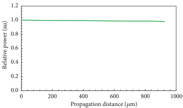
FIGURE 5: The total relative power throughout the proposed power splitter at \lambda = 1550 \text{ nm} .
