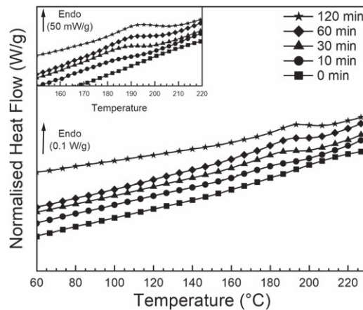
Figure 5. DSC thermograms recorded for bamboo strips after isothermal physical ageing at 160 °C for the times indicated on the figure. The framed details show a magnification of the Tg zone.
