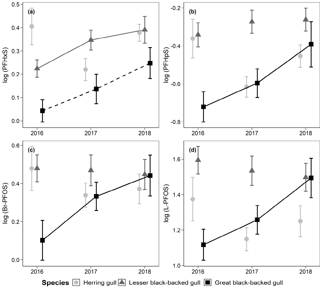
499 Figure 4: Error bar plots mean \pm standard error of sulfonate concentrations in 2016, 2017, and 2018 in the 500 seabird species from Ile de Re. The shapes and the three different grades of grey are used to distinguish the 501 three species as explained in the figure legend. Only significant trends are shown. Dashed lines indicate a 502 trend close to significance.
