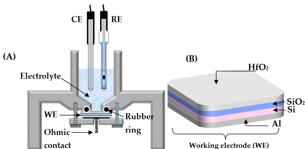
Figure 1. (A) Electrochemical cell used for pH measurement with Calomel-Saturated Reference electrode (RE), counter electrode (CE), and Ohmic contact behind the WE; (B) working electrode with electrolytic-insulating-semiconductor structure based on Al/Si/SiO 2 /HfO 2 .
