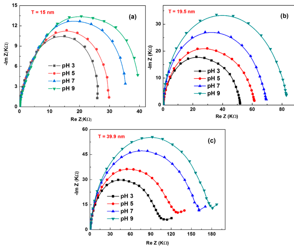
Figure 8. Nyquist plots at different pH for different hafnium thicknesses (a) 15.0 nm, (b) 19.5 nm and (c) 39.9 nm.
