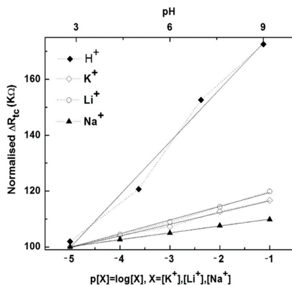
Figure 10. Calibration curve variation of normalized \Delta R_{tc} as a function of the pH versus (a) \text{K}^+ , (b) \text{Li}^+ and (c) \text{Na}^+ concentrations from 10^{-5} M to 10^{-1} M at the Si/SiO 2 /HfO 2 structure (thickness 39.9 nm).
