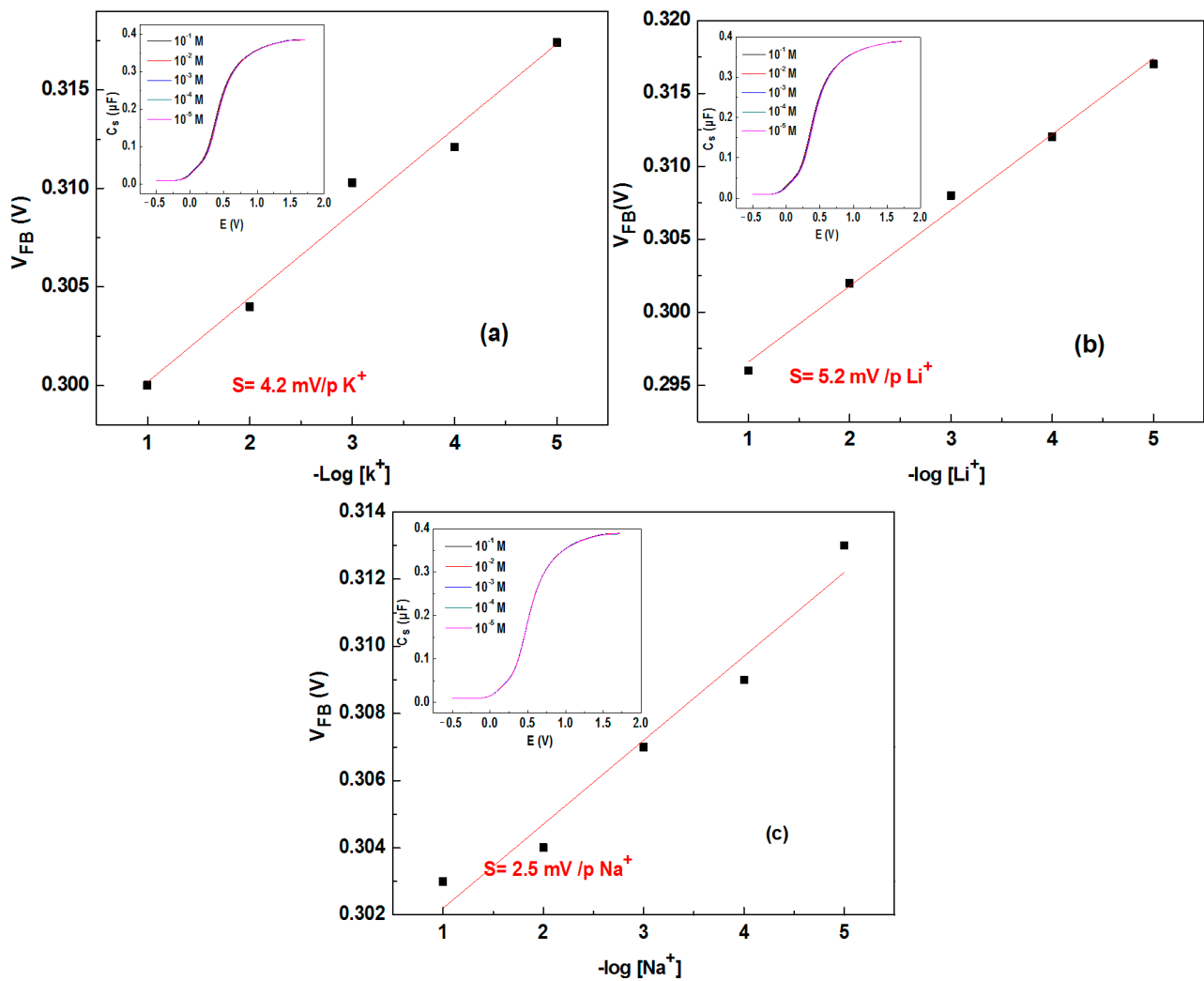
Figure 6. The flat band potential V_{FB} variation versus (a) K^+ , (b) Li^+ and (c) Na^+ concentrations from 10^{-5} M to 10^{-1} M. Inset: the capacitive responses of Si/SiO 2 /HfO 2 structure with 15 nm HfO 2 thickness for interfering ions (Figure S1 in Supplementary Material).
