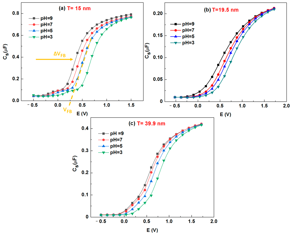
Figure 4. Typical C(V) curves for different hafnium thicknesses (a) 15.0 nm, (b) 19.5 nm and (c) 39.9 nm stacked \text{HfO}_2 structures for various pH buffer solutions using 0.4 M \text{Mg}(\text{NO}_3)_2 prepared in TRIS buffer. The pH was adjusted by the HCl solution ( C = 1 \text{ M} ).
