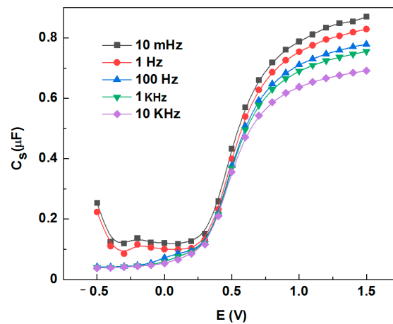
Figure 3. Typical C(V) response to frequency changes from 100 mHz to 100 kHz.
