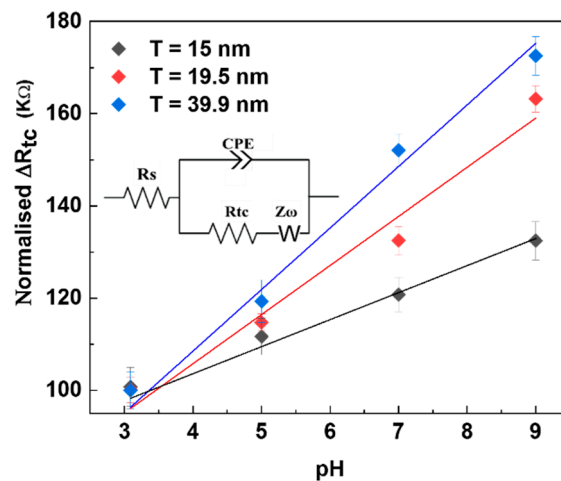
Figure 9. Calibration curve variation of normalized \Delta R_{ct} as a function of the pH for different hafnium oxide thickness of 15.0 nm, 19.5 nm and 39.9 nm.
