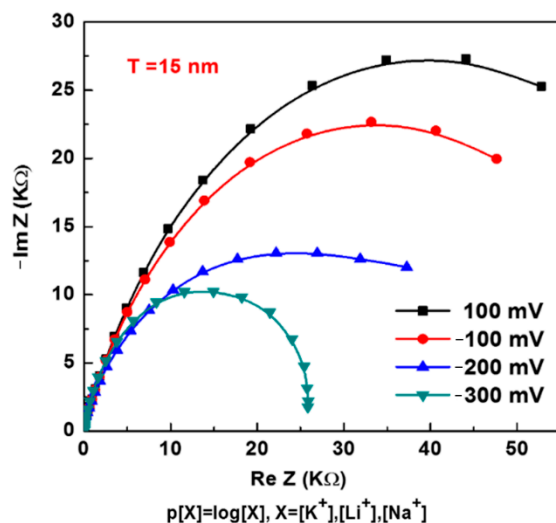
Figure 7. Impedance spectra (in Nyquist presentation) of the HfO 2 structures for different polarizations vs. saturated calomel reference electrode (SCE). Electrochemical impedance spectroscopy (EIS) measurements were carried out in 0.4 mol·L -1 Mg (NO 3 ) 2 prepared in TRIS buffer using the following conditions: frequency range from 100 mHz to 100 kHz, AC amplitude voltage at 25 mV.
