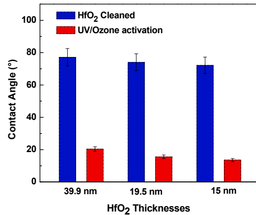
Figure 2. Contact angle measurements of the \text{HfO}_2 surface for the three thicknesses of 15.0, 19.5 and 39.9 nm used for the pH sensor based on \text{Al}/\text{Si}/\text{SiO}_2/\text{HfO}_2 .
