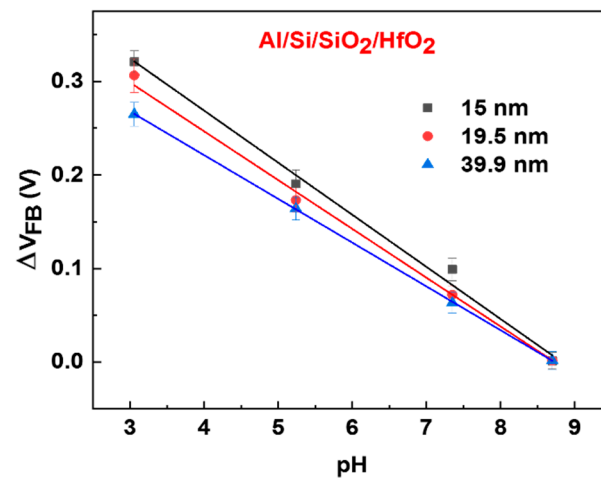
Figure 5. The pH sensitivity for three HfO 2 thicknesses (15.0, 19.5 and 39.9 nm): \Delta V_{FB} as a function of pH (from 3 to 9).
