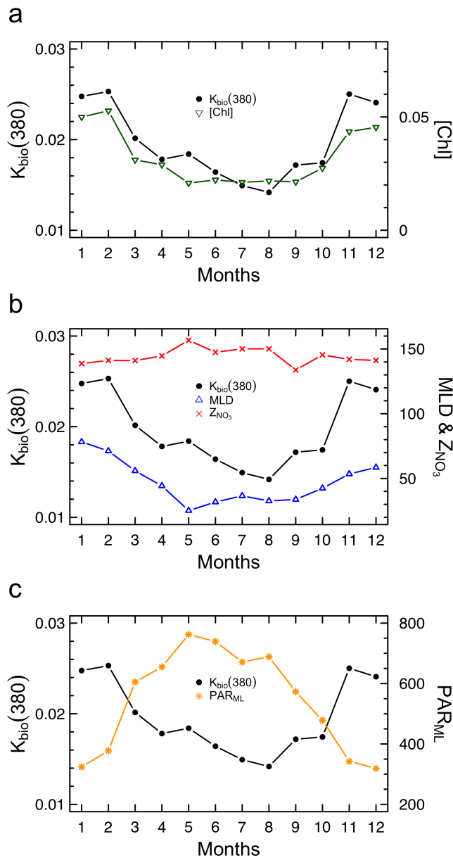
Figure 2. Monthly climatology of K_{bio}(380) (units of m^{-1} ) and other biogeochemical and physical variables within the mixed layer. (a) K_{bio}(380) and phytoplankton chlorophyll concentrations ([Chl]; units of milligrams per cubic meters); (b) K_{bio}(380) , the mixed layer depth (MLD; units of m) and the depth of the nitracline ( Z_{NO_3} ; units of m); (c) K_{bio}(380) and the average value of the Photosynthetically Available Radiation at solar noon within the mixed layer ( PAR_{ML} ; units of \mu mol\ quanta\ m^{-2}\ s^{-1} ). The coefficients of variation (CV%) for each monthly average are listed in Table S1.
