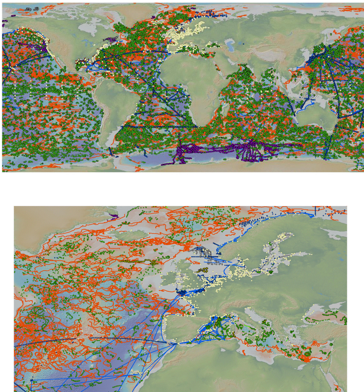
FIGURE 8 | Data at INS-TAC for Spring (January-March) 2018. Argo (green), vessels (XBT and CTD, thermosalinographs (blue), sea mammals (purple), gliders (yellow), moorings, tide gauges and rivers (white) (global and zoom on European seas).
