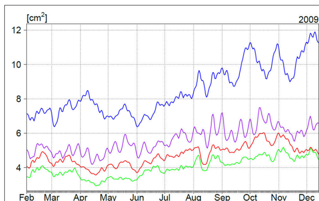
FIGURE 5 | Impact of a constellation of two wide-swath altimetry missions in a Northeast regional data assimilation system, for different constellation configurations and different instrumental error budgets (with reference to the SWOT Karin instrument) (Bonaduce et al., 2018). In that study, noise level requirements were less stringent as for Karin instrument. OSSE1 = 3 altimeters (SAR mode) (blue), OSSE2 = OSSE1 + Wide Swath (4 times Karin error) (violet), OSSE3 = OSSE1 + 2 Wide Swath (4 times Karin error) (red), OSSE4 = OSSE1 + 2 Wide Swath (2 times Karin error) (green). Units are in \text{cm}^2 . Results are given from February to December 2009.
