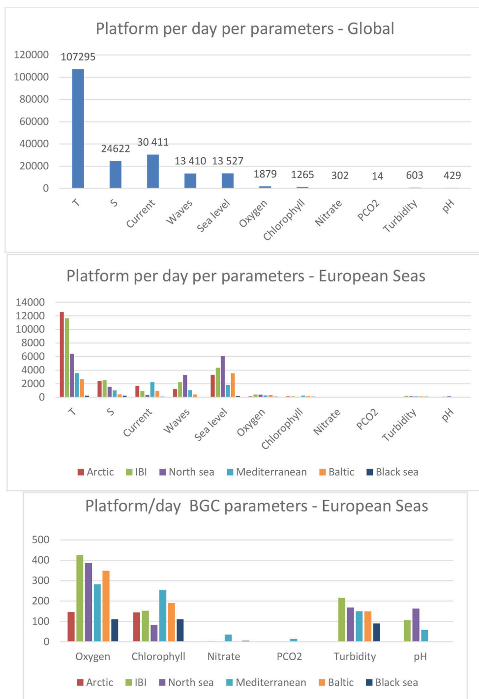
FIGURE 9 | Number of platforms providing observations per day (June 2018) by parameter (temperature, salinity, current, waves, sea level, oxygen, chlorophyll, nitrate, pCO 2 , turbidity, pH): (Top) global scale, (Middle) European seas (20N - 90N, 30W - 40E), and (Bottom) zoom on biogeochemical (BGC) data for the European seas.
