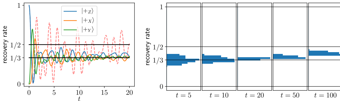
FIG. 4. Recovery ratio in a model of a qubit coupled to a semiclassical LMG model with spin S = 100 , J = 2.4 and \hbar = 2 . Left. Solid curves: Recovery ratio as function of time for three initial qubit states, when the bath is initialized to be maximally mixed. Dashed curve: the recovery ratio when the bath is initially a coherent (semiclassical) state with (X_c, Y_c, Z_c) \propto (1, 0, 0) [the qubit's initial state is |+z\rangle ]. We observe significant oscillation instead of a plateau. Right. Distribution of recovery ratio at t = 5, 10, 20, 50, 100 when the qubit initial state is randomly and uniformly chosen on the Bloch sphere. 300 samples are calculated for each histogram.
