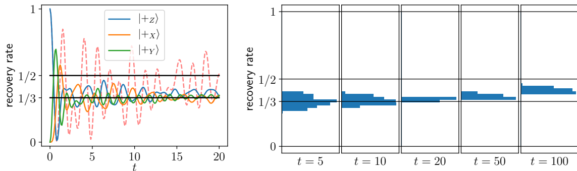
FIG. 4. Recovery ratio in a model of a qubit coupled to a semiclassical LMG model with spin S = 100 , J = 2.4 and \hbar = 2 . Left . Solid curves: Recovery ratio as function of time for three initial qubit states, when the bath is initialized to be maximally mixed. Dashed curve: the recovery ratio when the bath is initially a coherent (semiclassical) state with (X_c, Y_c, Z_c) \propto (1, 0, 0) [the qubit's initial state is |+z\rangle ]. We observe significant oscillation instead of a plateau. Right . Distribution of recovery ratio at t = 5, 10, 20, 50, 100 when the qubit initial state is randomly and uniformly chosen on the Bloch sphere. 300 samples are calculated for each histogram.
