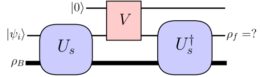
FIG. 1. The information recovery process under consideration. The information \psi_i stored in a qudit (middle) is encoded by a scrambler U_s which couples the qudit to a bath (bottom). The information can be decoded by applying the time-reversed evolution, U_s^\dagger . What is the effect of an eavesdropping action (i.e. coupling with an ancilla qubit (top) by unitary operator V ) ?
