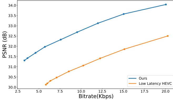
Fig. 2: RD curve for 90 test videos sampled from VoxCeleb test set encoded by our framework.
