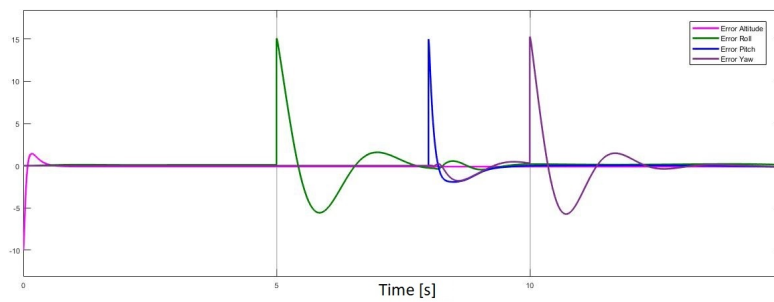
Fig. 9: Error signals.
