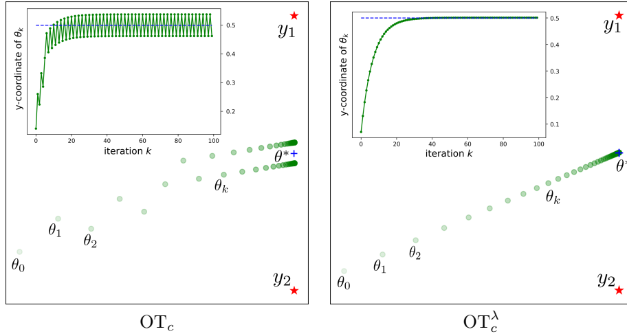
Figure 1: Plot of the trajectory of the parameter \theta^k during optimization of the generative model g_\theta(z) = z - \theta for two training points \{y_1, y_2\} . Left: as predicted by Proposition 1, the process does not converge for the optimal transport \text{OT}_c with quadratic cost c = \|\cdot\|^2 . Right: as supported by Theorem 5, the training converges to the solution \theta^* = (0, 0.5) when considering regularized optimal transport \text{OT}_c^\lambda . See Section 3.4 for more details.
