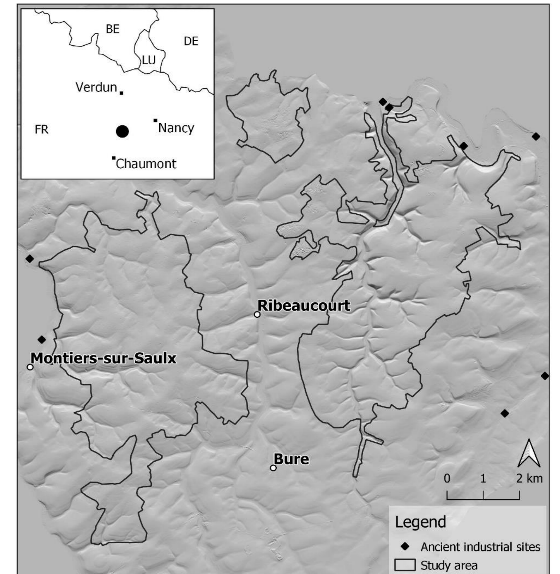
Fig. 2 | Study area in southern Meuse (NE France). The forest patches (black contour, 57.3km 2 ) and ancient industrial activities (smithies) displayed in the LiDAR-derived Digital Elevation Model.
