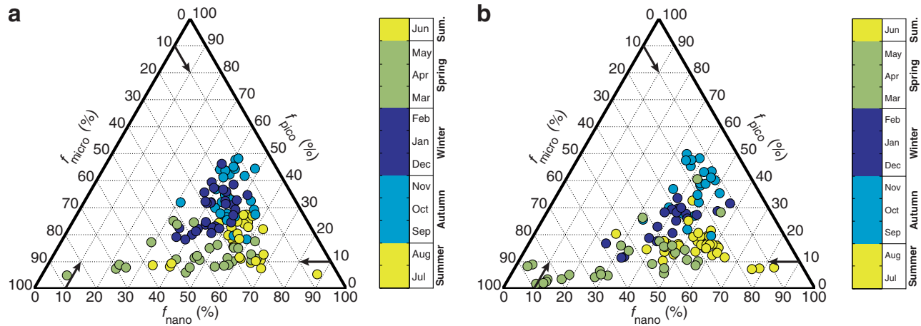
Figure 6. Ternary plots of the climatological seasonal variations between 0 m and 1.5 \times Z_{eu} of the fraction of the [Chl-a] associated with the three phytoplankton size classes: micro ( f_{micro} ), nano ( f_{nano} ), and pico-phytoplankton ( f_{pico} ), for the two studied trophic regimes: (a) "Bloom" and (b) "High Bloom", at the DYFAMED/BOUSSOLE site. Each color represents a season.
