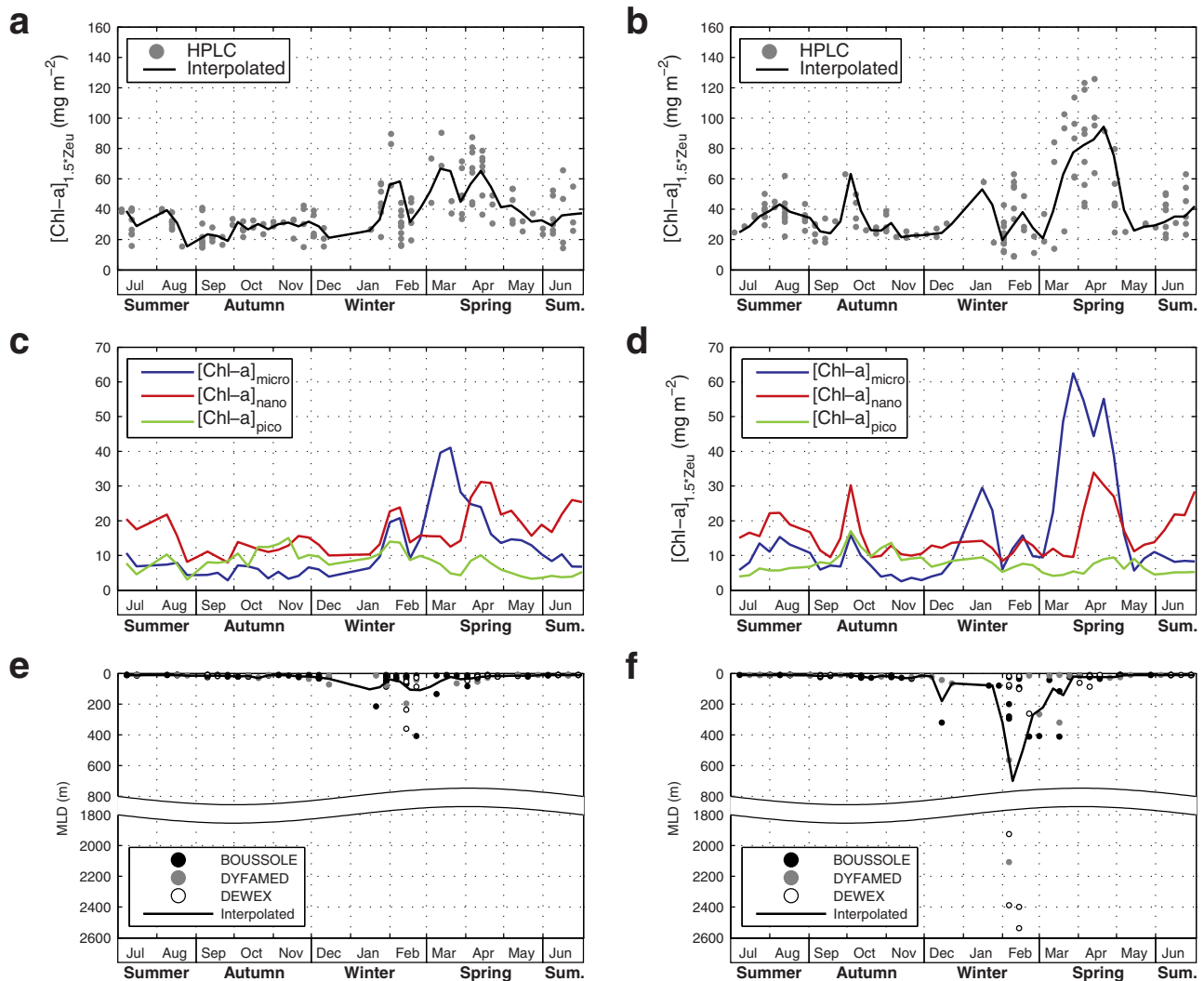
Figure 7. Climatological annual cycle of total and class-specific [Chl-a]_{1.5 \times Z_{eu}} and of the MLD, for the two studied trophic regimes: (a, c, e) "Bloom" and (b, d, f) "High Bloom." The total [Chl-a]_{1.5 \times Z_{eu}} is the sum of each (c, d) class-specific [Chl-a]_{1.5 \times Z_{eu}} : [Chl-a]_{micro} , [Chl-a]_{nano} , and [Chl-a]_{pico} (for the micro, nano, and pico-phytoplankton, respectively). (e, f) For the BOUSSOLE project (black points), the maximum possible MLD value is 400 m (the greatest depth of the CTD cast).
