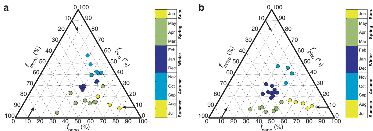
Figure 4. Ternary plots of the seasonal variations between 0 m and 1.5 \times Z_{eu} of the fraction of [Chl- a ] associated with the three phytoplankton size classes: micro ( f_{micro} ), nano ( f_{nano} ), and pico-phytoplankton ( f_{pico} ), for the two studied trophic regimes: (a) “Bloom” and (b) “High Bloom”, between July 2012 and July 2013 (DEWEX cruises). Each color represents a season.
