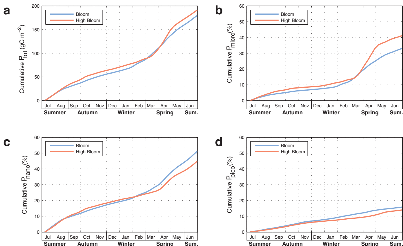
Figure 9. Climatological annual cycle of cumulative total and class-specific primary production for the two studied trophic regimes obtained from the light photosynthesis model. Each class-specific primary production: (b) P_{micro} , (c) P_{nano} , and (d) P_{pico} (for the micro, nano, and pico-phytoplankton, respectively), is expressed in percentage of (a) the total primary production ( P_{tot} ).
