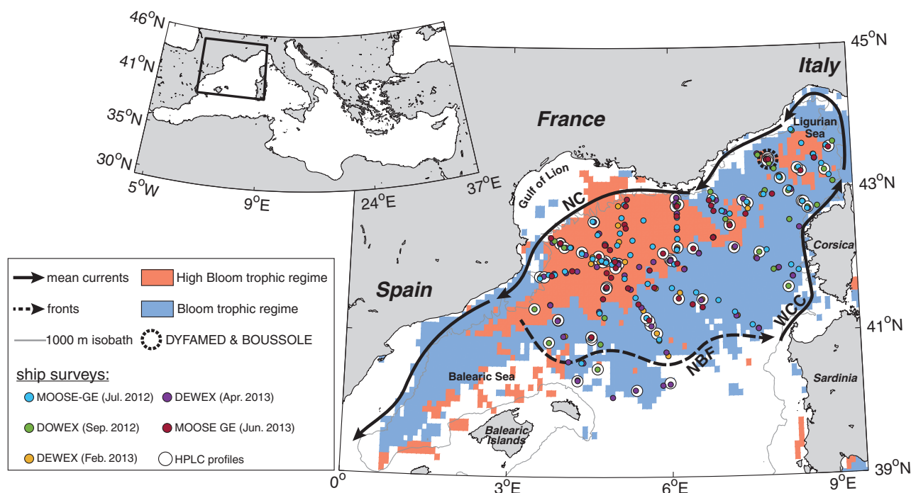
Figure 1. Map of the NWM showing the location of cruise stations and of the DYFAMED/BOUSSOLE site. Colored areas indicate the spatial location of the two studied trophic regimes in 2012/2013 (the “Bloom” and “High Bloom” trophic regimes, from Mayot et al. [2016a]). The mean currents are represented by arrows with continuous lines (WCC: Western Corsican Current, NC: Northern Current) and the North Balearic Front (NBF) by an arrow with a dashed line.
