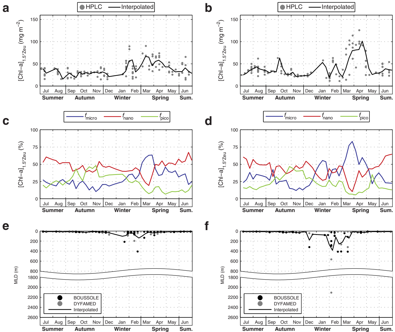
Figure 5. Climatological annual cycle of total and class-specific [Chl-a]_{1.5*Zeu} and of the MLD, for the two studied trophic regimes: (a, c, e) “Bloom” and (b, d, f) “High Bloom” at the DYFAMED/BOUSSOLE site. The total [Chl-a]_{1.5*Zeu} is the sum of each (c, d) class-specific [Chl-a]_{1.5*Zeu} : [Chl-a]_{micro} , [Chl-a]_{nano} and [Chl-a]_{pico} (for the micro, nano and pico-phytoplankton, respectively). (e, f) For the BOUSSOLE project (black points), the maximum possible MLD value is 400 m (the greatest depth of the CTD cast).
