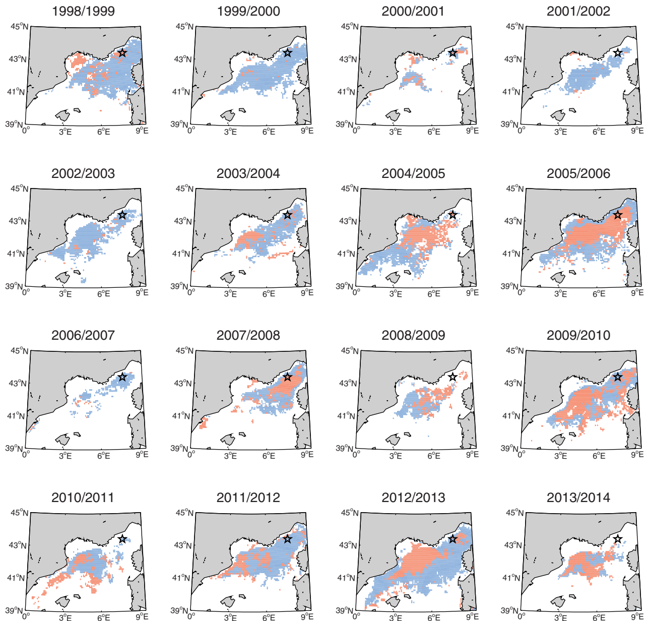
Figure 2. Spatial extent of the “Bloom” (blue) and “High Bloom” (orange) trophic regimes in the NWM and for the years indicated [from Mayot et al. , 2016a]. The year is here defined between July and July (e.g., for 1998/1999: July 1998 to July 1999). The star in the Ligurian Sea indicates the location of the DYFAMED/BOUSSOLE site.
