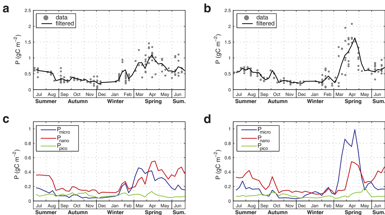
Figure 8. Climatological annual cycle of total and class-specific daily primary production for the two studied trophic regimes, obtained from the light photosynthesis model. (a, b) The total primary production is the sum of (c, d) each class-specific primary production: P_{\text{micro}} , P_{\text{nano}} , and P_{\text{pico}} (for the micro, nano, and pico-phytoplankton, respectively). These results are displayed separately for the (a, c) “Bloom” and (b, d) “High Bloom” trophic regimes.
