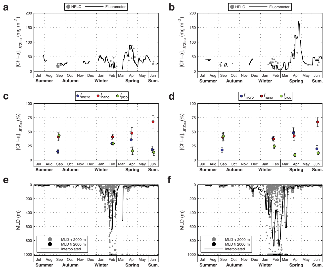
Figure 3. Annual cycle of total and class-specific [\text{Chl-a}]_{1.5\text{ZeU}} and of the MLD, for the two studied trophic regimes: (a, c, e) “Bloom” and (b, d, f) “High Bloom” between July 2012 and July 2013 (DEWEX cruises). The total [\text{Chl-a}]_{1.5\text{ZeU}} is the sum of each (c, d) class-specific [\text{Chl-a}]_{1.5\text{ZeU}} : [\text{Chl-a}]_{\text{micro}} , [\text{Chl-a}]_{\text{nano}} , and [\text{Chl-a}]_{\text{pico}} (for the micro, nano, and pico-phytoplankton, respectively). The total [\text{Chl-a}]_{1.5\text{ZeU}} was also obtained from fluorometers measurements (black lines). (c, d) The mean class-specific [\text{Chl-a}]_{1.5\text{ZeU}} (with the standard deviation) is calculated for each DEWEX cruises (Table 1). (e, f) The MLD estimations higher or equal to 2000 m are indicated by black dots.
