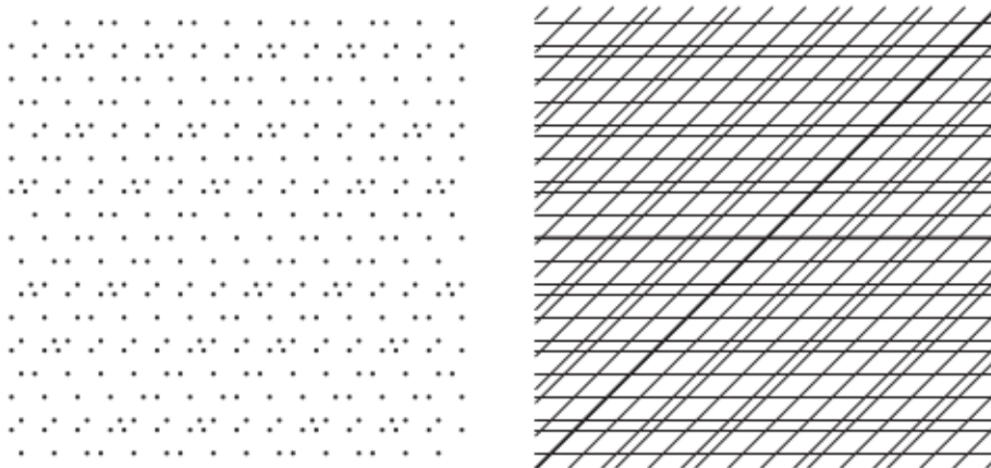
Fig. 3. The \delta -lattice I_1(\delta) with points (left), and its trivial tiling obtained by joining points along the horizontal axis, and along the direction defined by \zeta .
