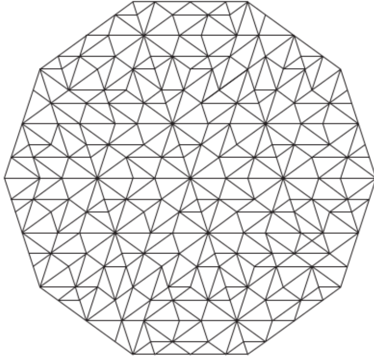
Fig. 1. A tiling of the \tau -lattice F_1(\tau) .
