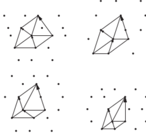
Fig. 6. Rotation operator r_1 applied to elementary tiles of the \tau -lattice I_1(\tau) , \mathbf{T}(0) , \mathbf{T}(1) (up), \mathbf{T}(\zeta) and \mathbf{T}(1 + \zeta) (down). Note how the tiles are deformed, by this operation, in order for the vertices to remain in I_1(\tau) . The arrows indicate the vertices of the new tile in which are mapped the vertices of the original tile.
