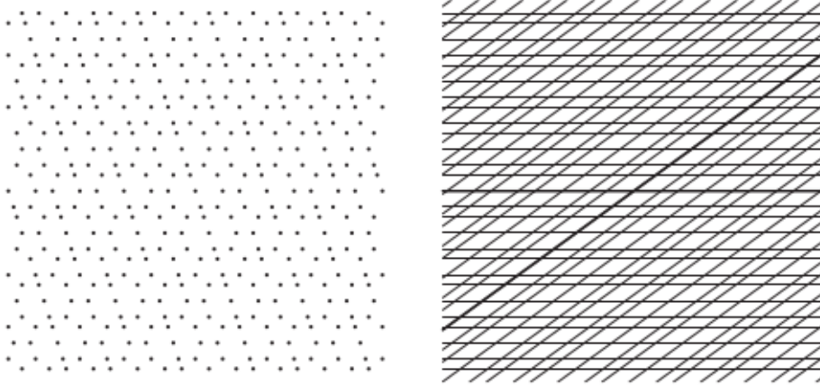
Fig. 2. The \tau -lattice I_1(\tau) with points (left), and its trivial tiling made by joining points along the horizontal axis, and along the direction defined by \zeta .
