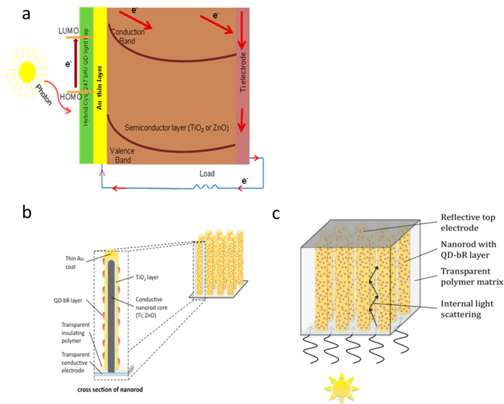
Figure 1. (a) Planar structure of the solid-state photovoltaic device. (b) Illustration of a nanowire array showing the conductive core, covered, respectively, by \text{TiO}_2 (or \text{ZnO} ) semiconductor metal oxides, Au, and QD-bR dye layers. Panel c illustrates how the nanowire array can be packaged to include a lower transparent electrode, a transparent polymer matrix to provide mechanical stability and flexibility, and a top reflective electrode. The polymer matrix can include particles with index of refraction differing from the matrix to further enhance internal reflections.
