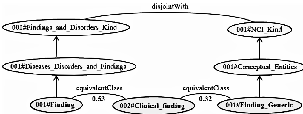
Figure 7: Two Ambiguous Equivalence Correspondences Leading to Unsatisfiable Classes in a Simple-Merge Ontology (or Leading to an Unsatisfiable Class in a Full-Merge Ontology)
