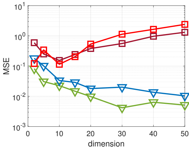
Fig. 2. Example V-B. MSE in the estimation of E_{\tilde{\pi}}[\mathbf{X}] of the banana-shaped distribution versus the dimension d_x , with GR-PMC (brown square), LR-PMC (red square) with \sigma = 1 , and the proposed O-PMC method with LR (green triangle) or GLR (blue triangle) schemes.
