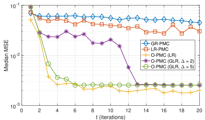
Fig. 3. Example V-C. Evolution of the median MSE with respect to ground truth amplitudes and frequencies for dimension d_x = 4 as function of the number of iterations of GR-PMC, LR-PMC, and O-PMC.
