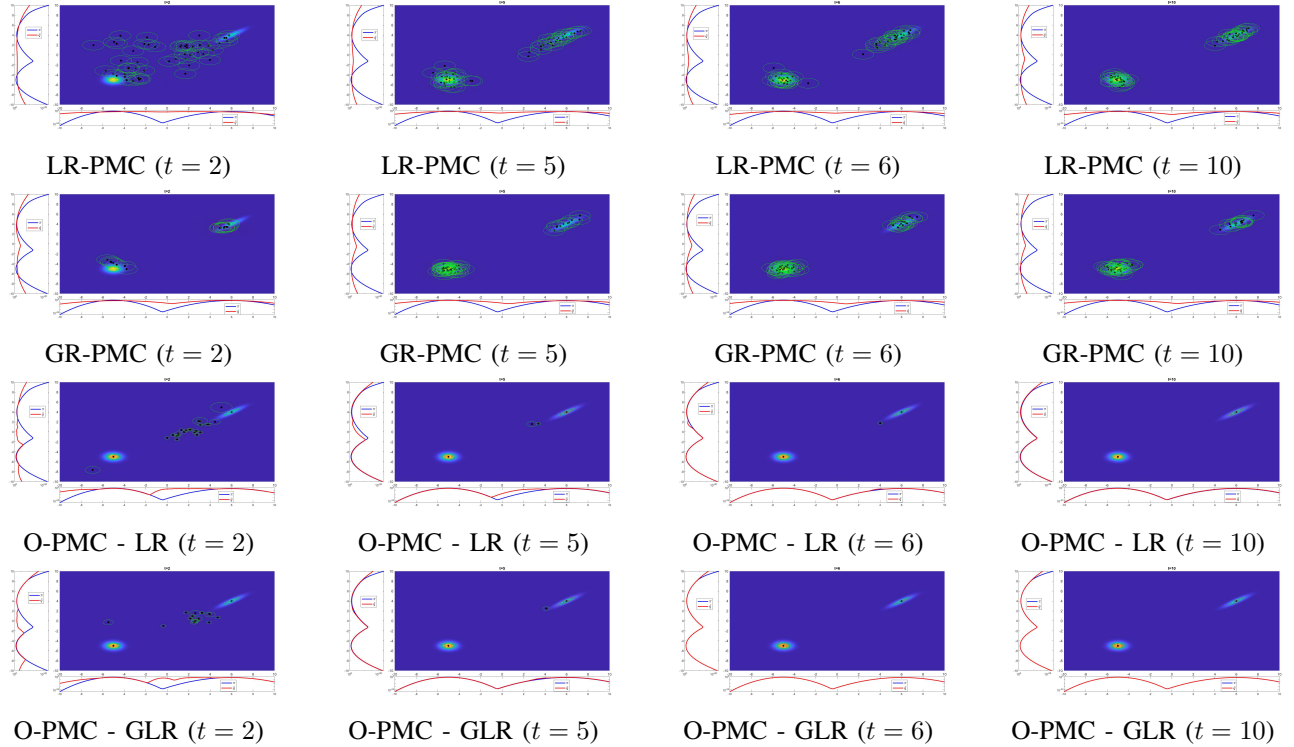
Fig. 1. Toy example. Evolution of the reconstructed target along iterations for LR-PMC, GR-PMC and O-PMC for both LR and GLR (with \Delta = 5 ). One can notice the fast convergence of the proposed O-PMC. The great impact of GLR can be seen, by comparing both O-PMC variants (LR / GLR) between time t = 5 to time t = 6 , i.e. after and before applying the GR step in the GLR approach.
