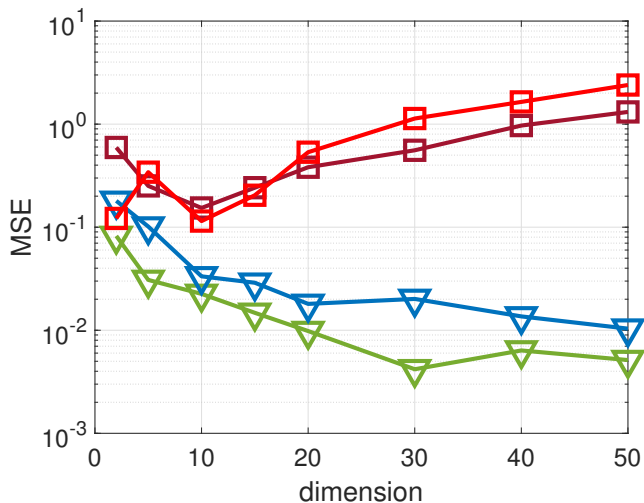
Fig. 2. Example V-B. MSE in the estimation of E_{\pi}[\mathbf{X}] of the banana-shaped distribution versus the dimension d_x , with GR-PMC (brown square), LR-PMC (red square) with \sigma = 1 , and the proposed O-PMC method with LR (green triangle) or GLR (blue triangle) schemes.
