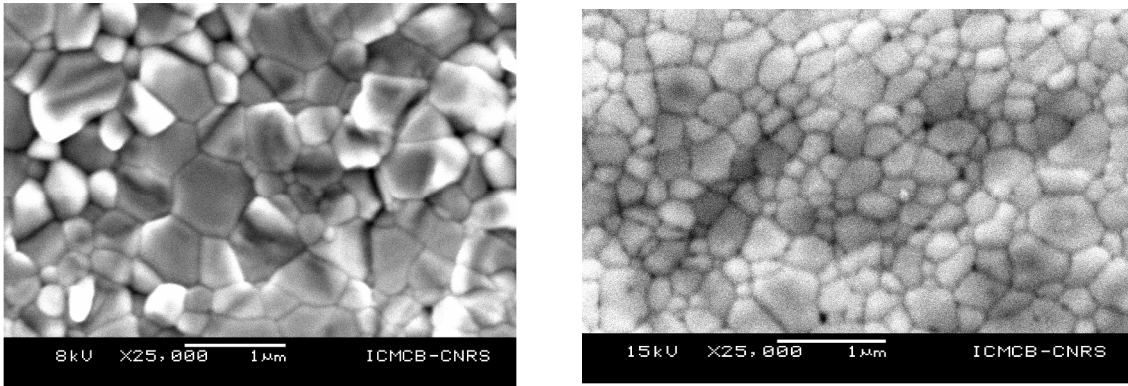
Fig (a) SEM micrographs of YLO ceramics (b) 500°C, 100 MPa, t_s=5 min and R_H=50^\circ\text{C}/\text{min} , annealed at 1200°C for 12 h (b) 1700°C, 100 MPa, t_s=5 min and R_H=50^\circ\text{C}/\text{min} , annealed at 1200°C for 12 h
