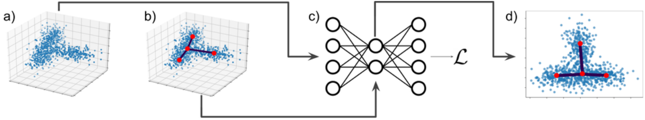
Figure 1: Schematic method overview. a) High-dimensional data. b) Proposed density tree. After computing the k -means centroids on the data, we build a tree based on the data density between pairs of centroids. c) DTAE. An autoencoder is used to learn a representation of our data. This embedding is regularized by the previously computed tree in order to preserve its hierarchical structure in low-dimensional space. d) The final DTAE embedding. After training of the autoencoder, the bottleneck layer visualizes the data in low dimension and respects the density structure.
