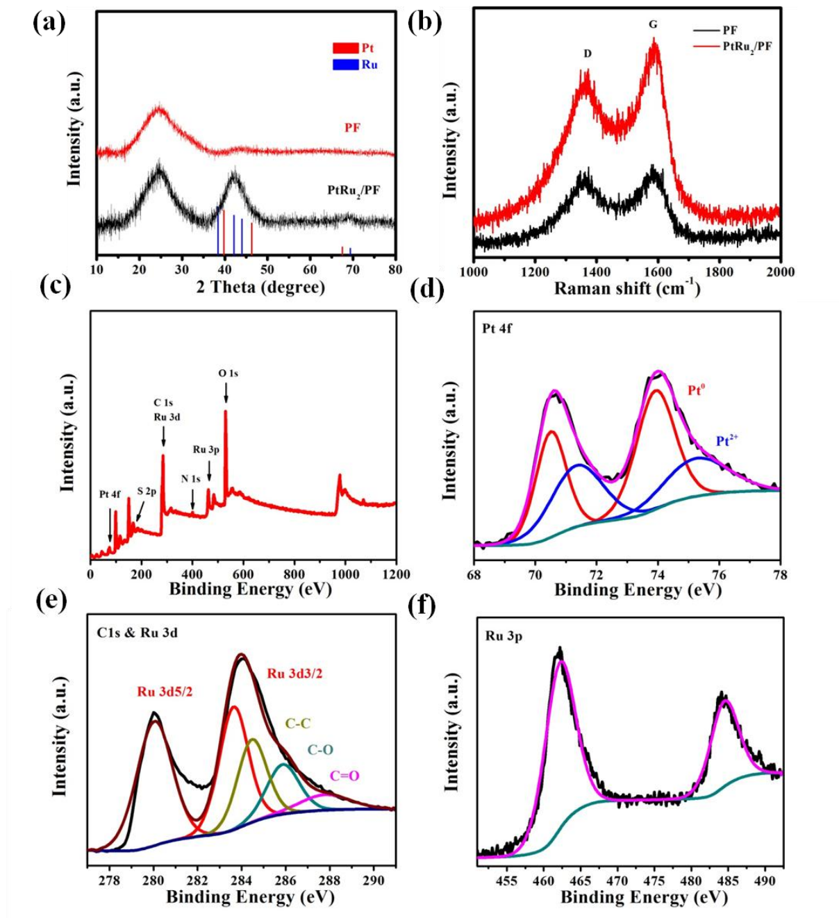
Figure 3. (a) XRD patterns, and (b) Raman spectra of PF and PtRu 2 /PF. (c) XPS full scan and core level spectra of (d) Pt 4f, (e) C 1s and Ru 3d, and (f) Ru 3p of PtRu 2 /PF.
