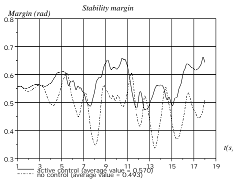
Figure 7: results of the stability control algorithms
