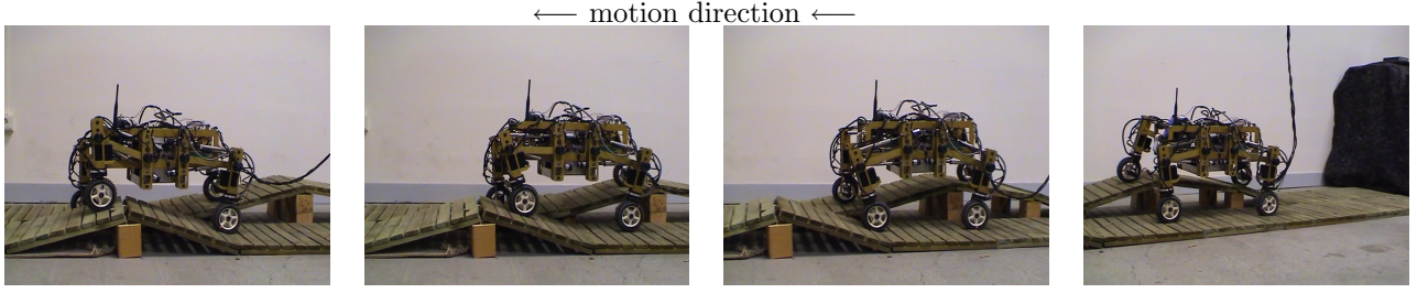
Figure 3: Hyl0s 1 evolving on an irregular ground profile with a constant nominal configuration (Mode 2).
