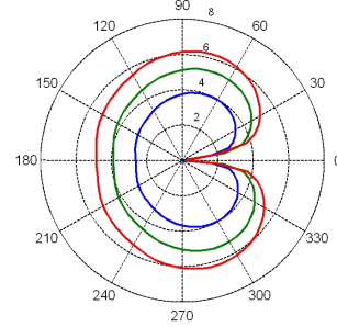
Fig. 5: Boat-specific polar diagram.
