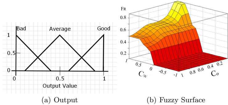
Fig. 7: Output fuzzy sets and surface
