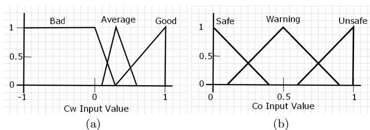
Fig. 6: Fuzzy system for heading selection
